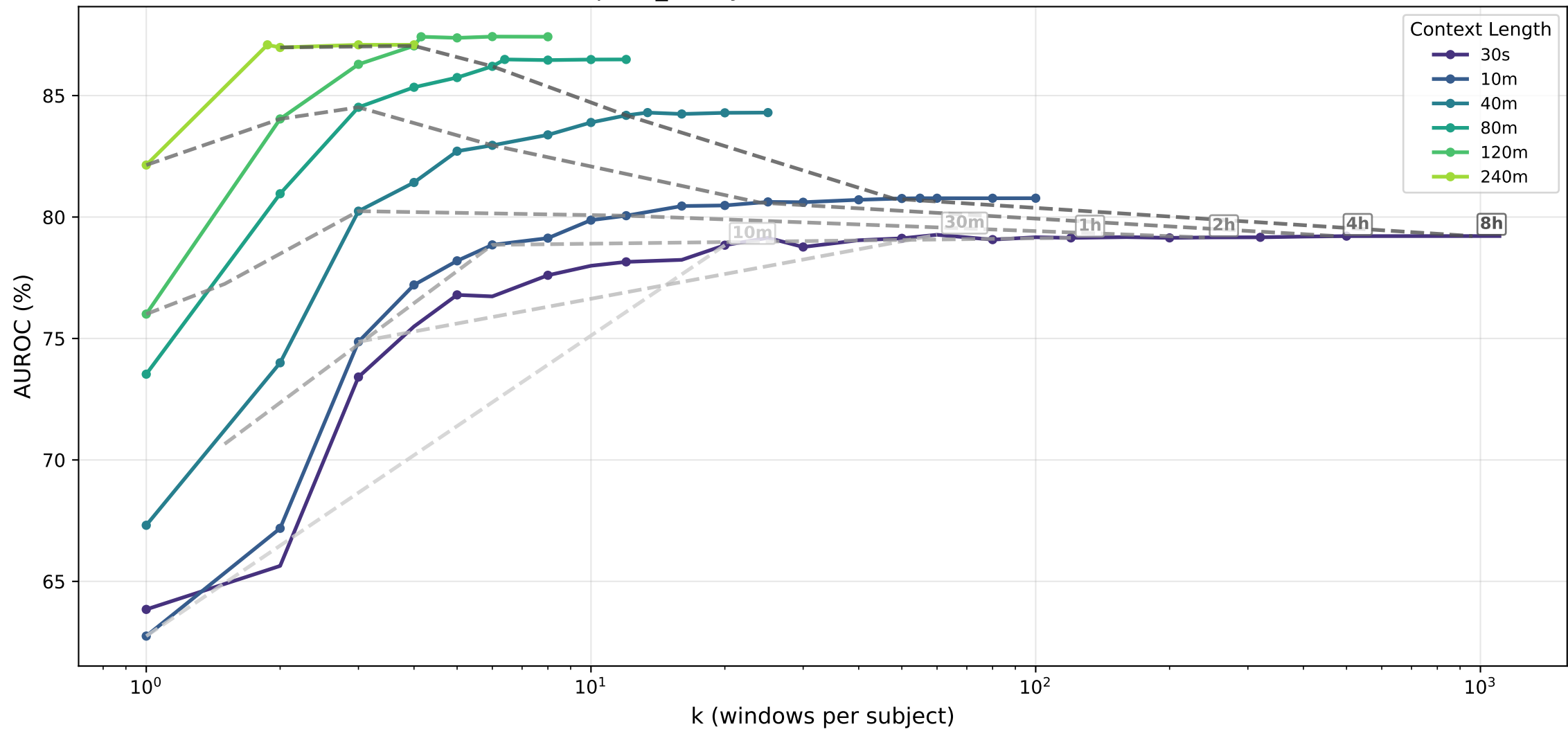
apnea_binary · lstm — AUROC (%) vs k
