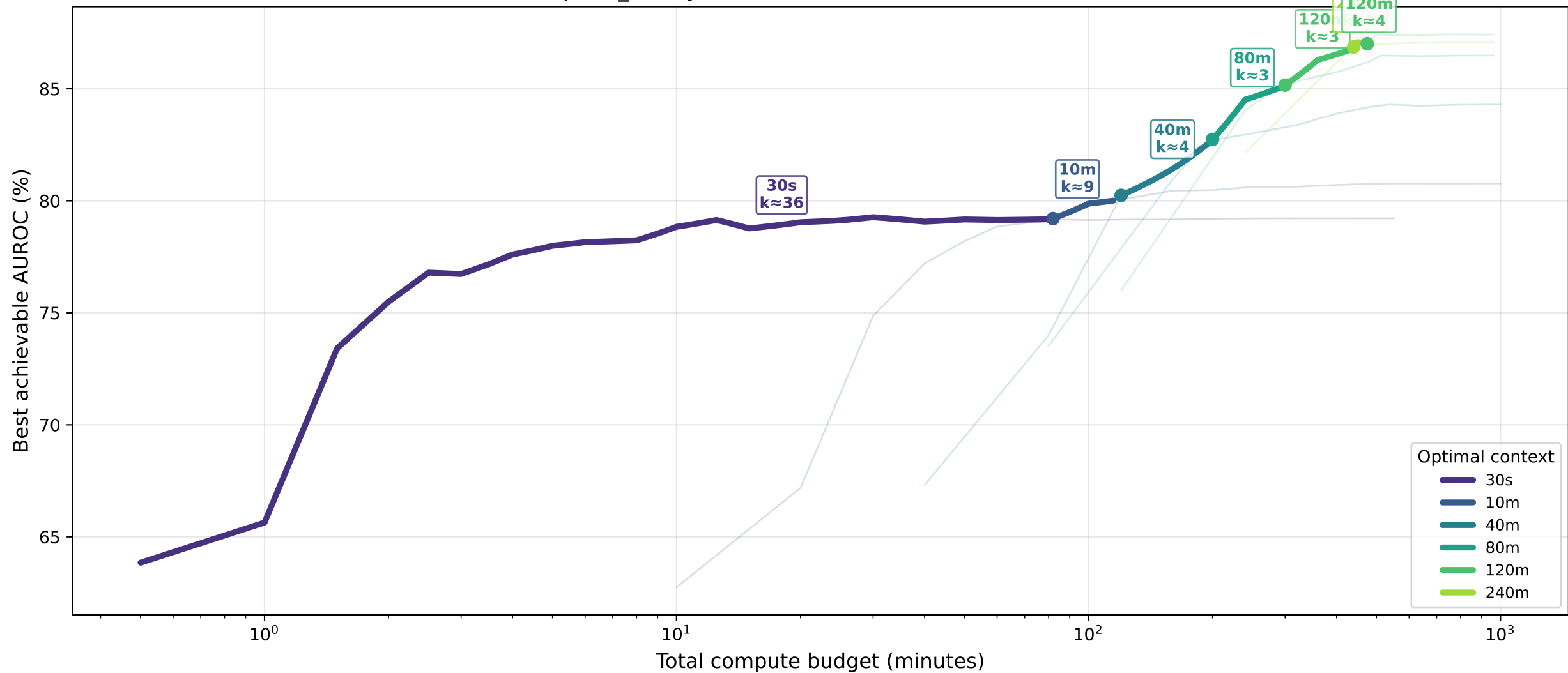
apnea_binary · Istm — Pareto Front: AUROC (%)
