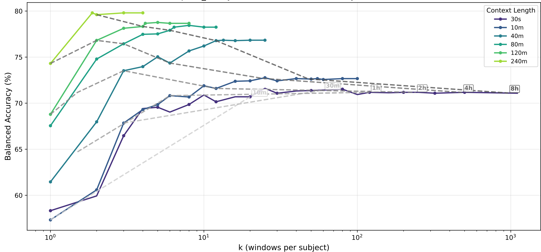
apnea_binary · lstm — Balanced Accuracy (%) vs k
