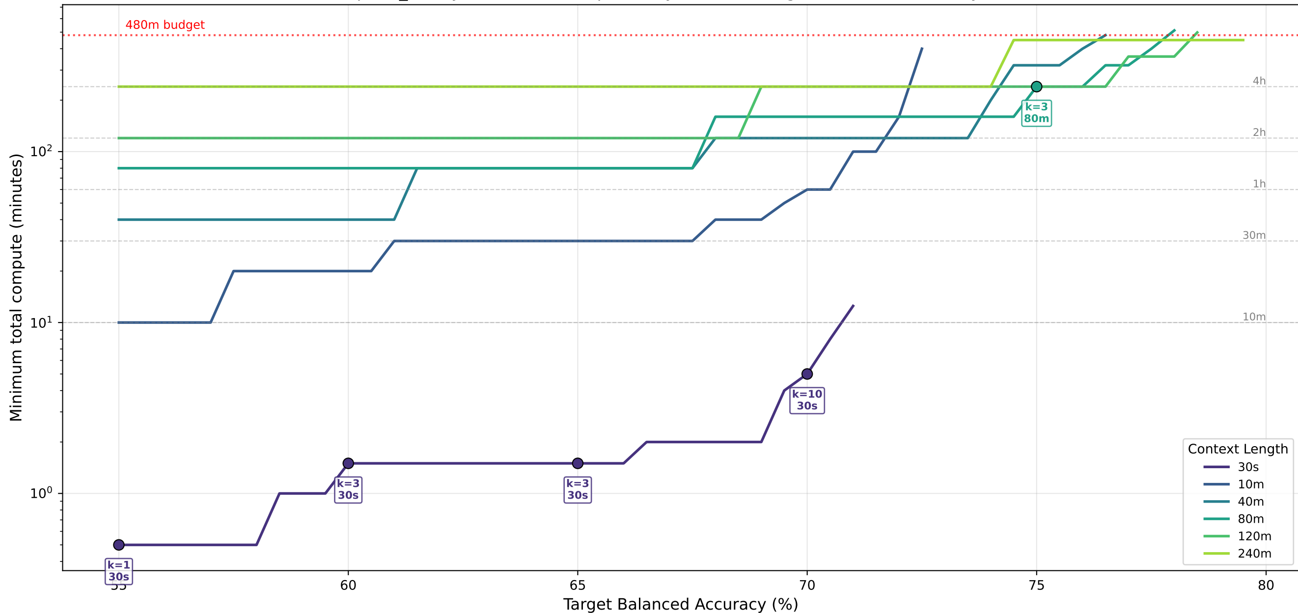
apnea_binary · lstm — Cheapest Way to Reach Target Balanced Accuracy (%)
