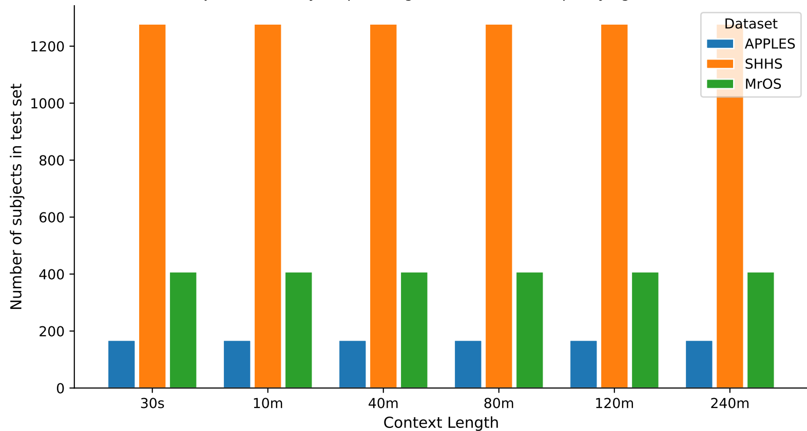
Test-Set Subject Count per Dataset — apnea_binary (TRANSFORMER) Subject count may drop at longer contexts (fewer qualifying windows)
