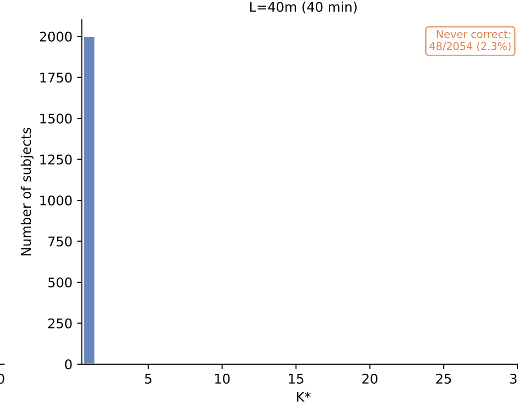
K* Distribution — apnea_binary (TRANSFORMER) K* = minimum windows for correct classification (reps=20)
