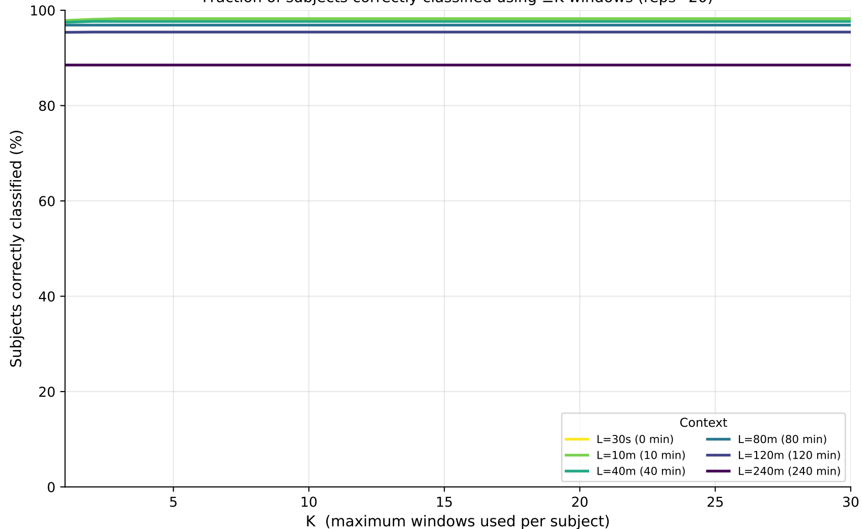
Coverage Curves — apnea_binary (TRANSFORMER) Fraction of subjects correctly classified using \leq K windows (reps=20)
