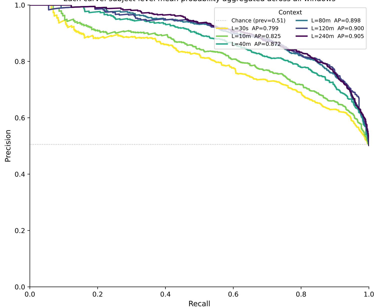
Precision-Recall Curves — apnea_binary (TRANSFORMER) K=all Each curve: subject-level mean probability aggregated across all windows
