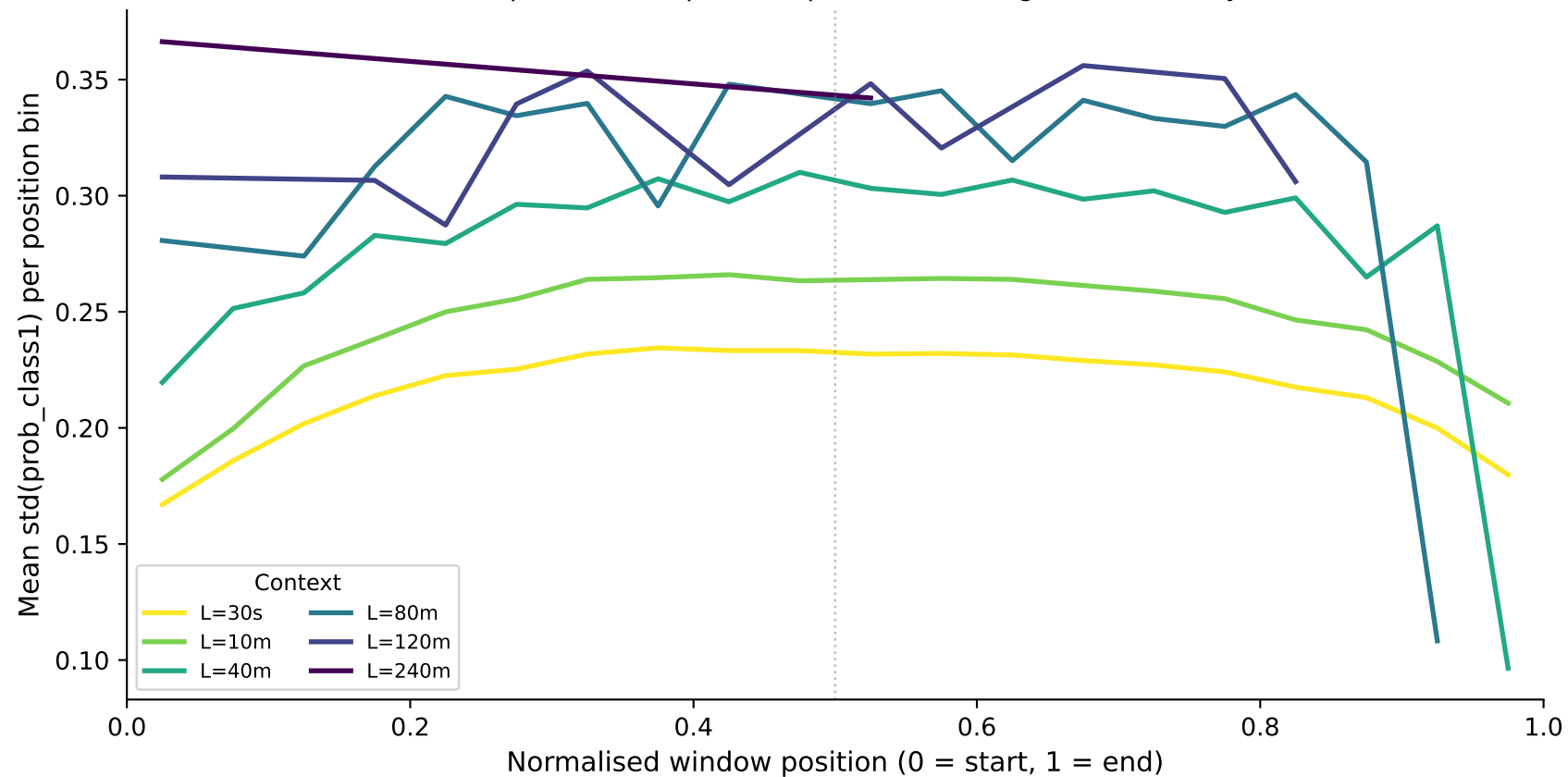
Prediction Variance vs Night Position — apnea_binary (TRANSFORMER) Lower variance = position-independent predictions (longer context may flatten this)
