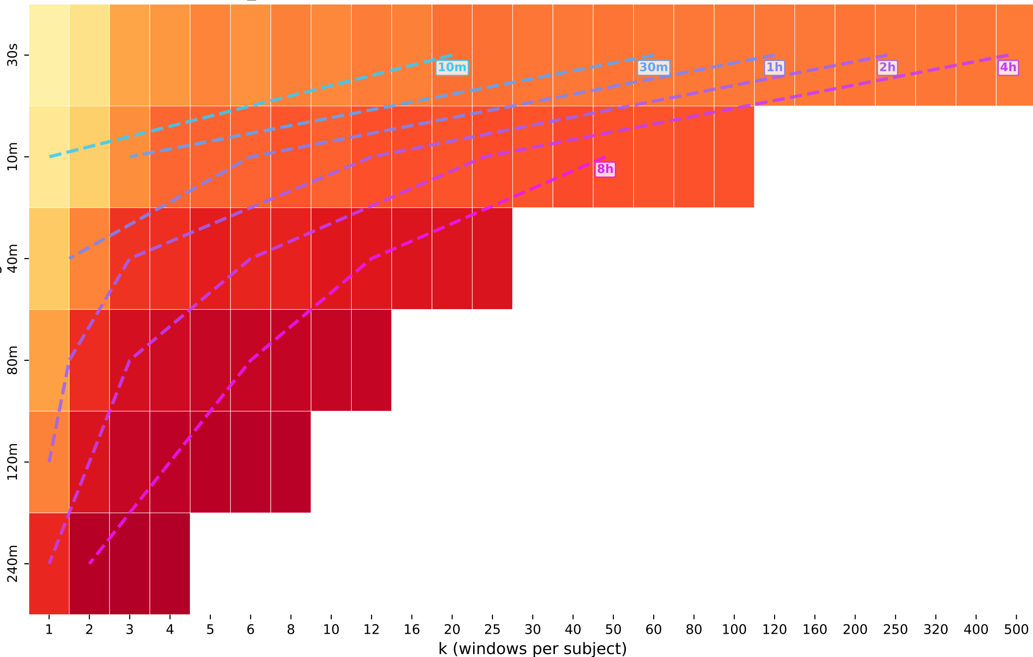
apnea_binary · transformer — Iso-Compute Heatmap: Balanced Accuracy (%)
