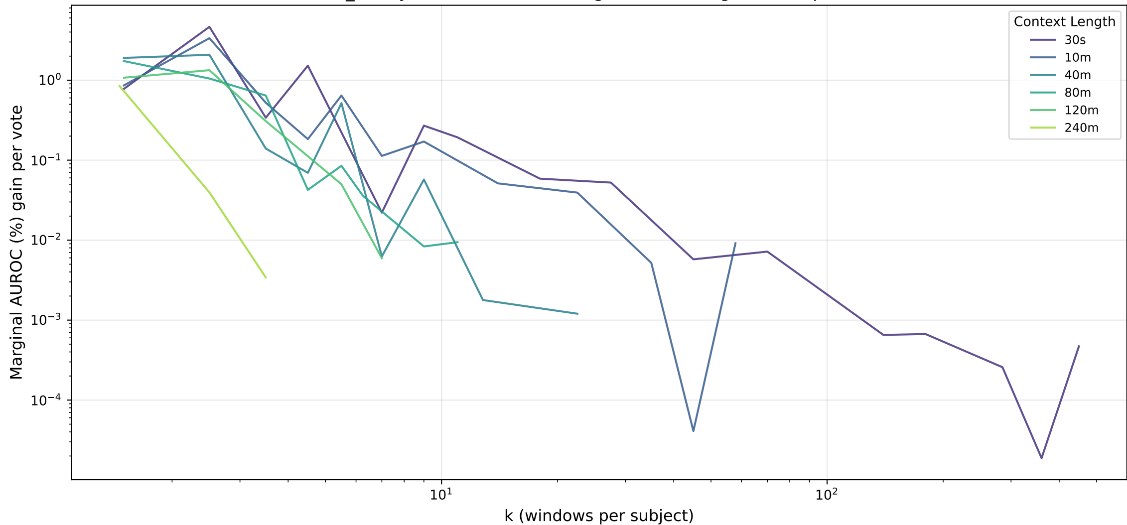
bmi_binary · Istm — Diminishing Returns: Marginal Gain per Vote
