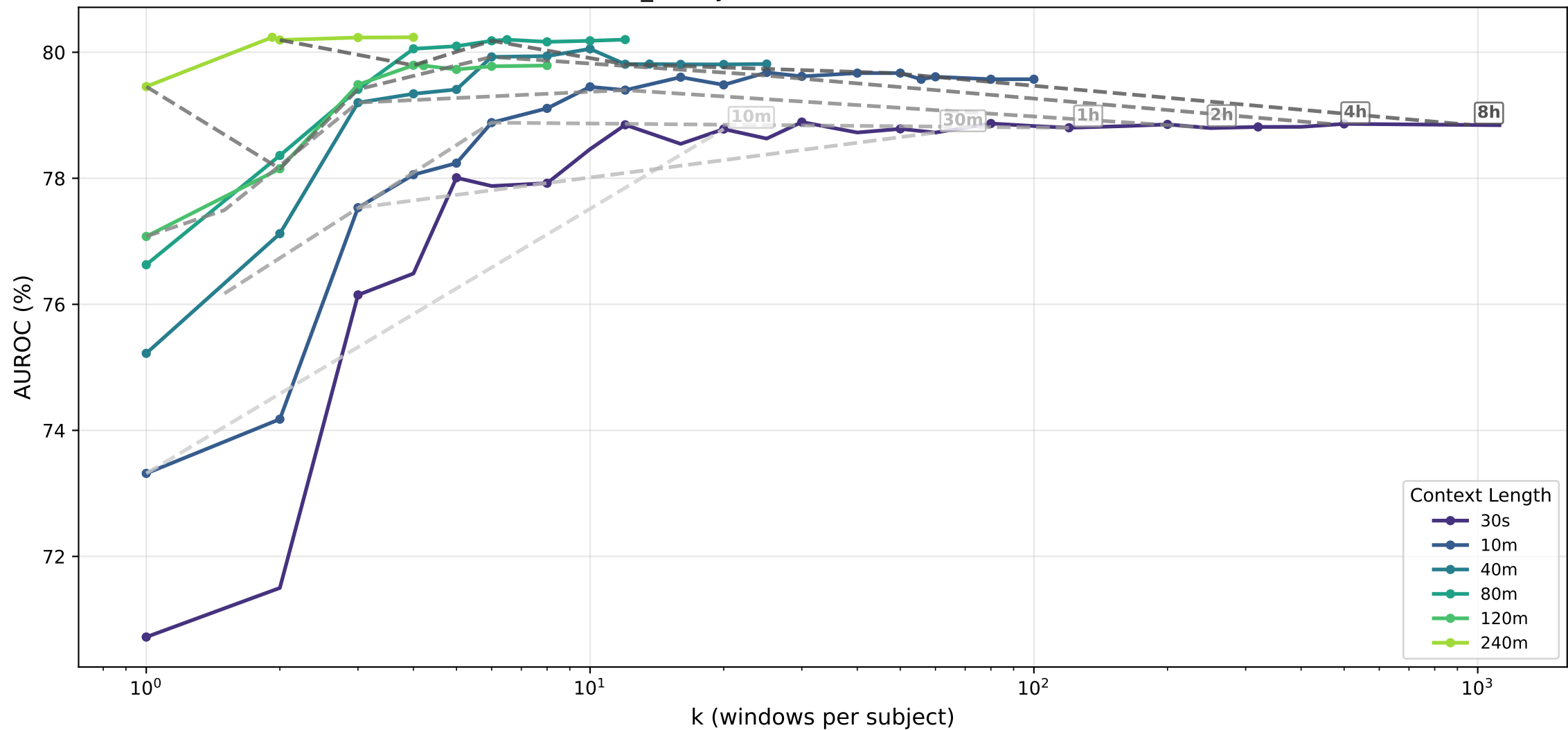
bmi_binary · lstm — AUROC (%) vs k
