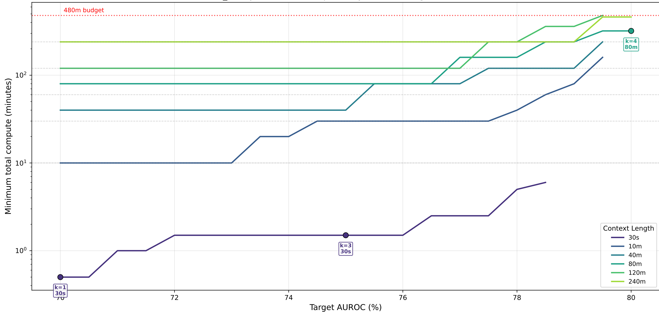
bmi_binary · lstm — Cheapest Way to Reach Target AUROC (%)
