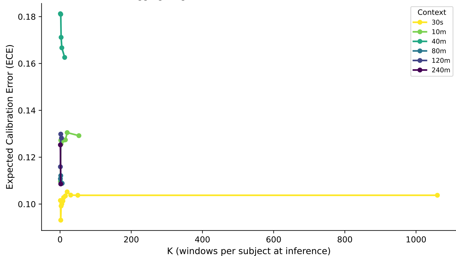
ECE vs K — bmi_binary (LSTM) Aggregating more windows reduces calibration error
