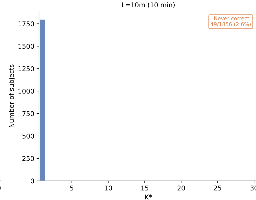
K* Distribution — bmi_binary (LSTM) K* = minimum windows for correct classification (reps=20)
