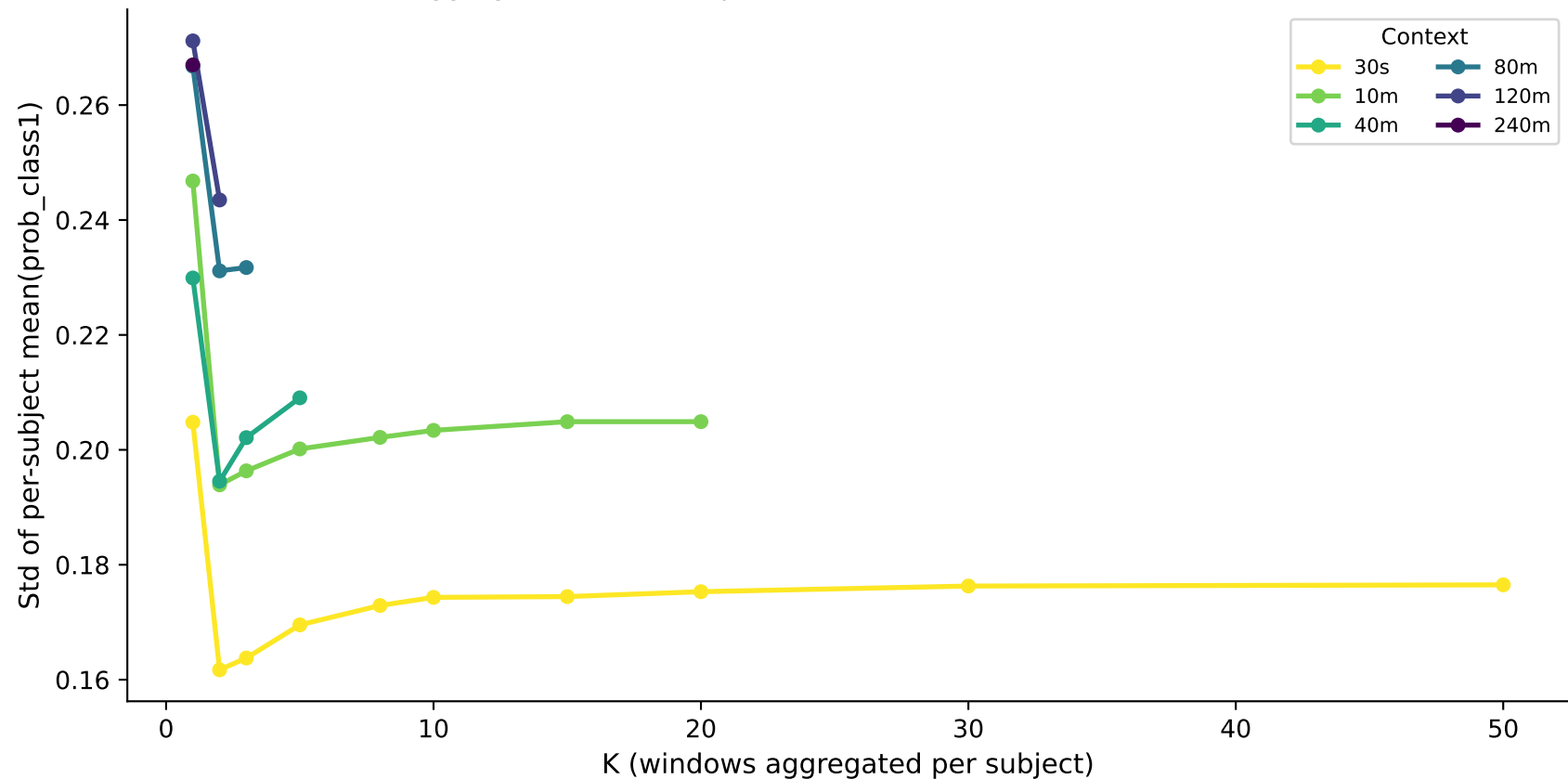
Prediction Variance vs K — bmi_binary (LSTM) Aggregation stabilises predictions (lower std = more consistent)
