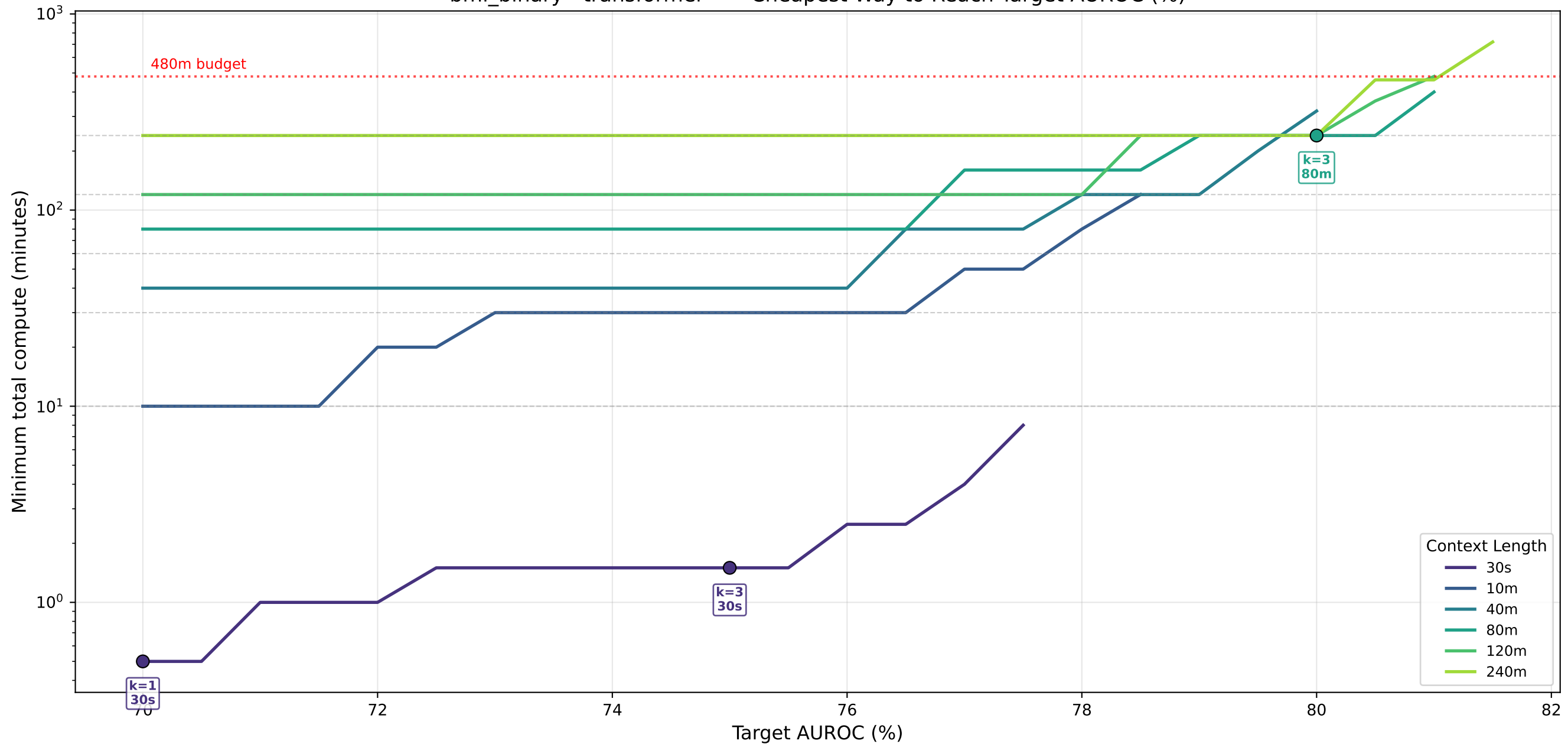
bmi_binary · transformer — Cheapest Way to Reach Target AUROC (%)
