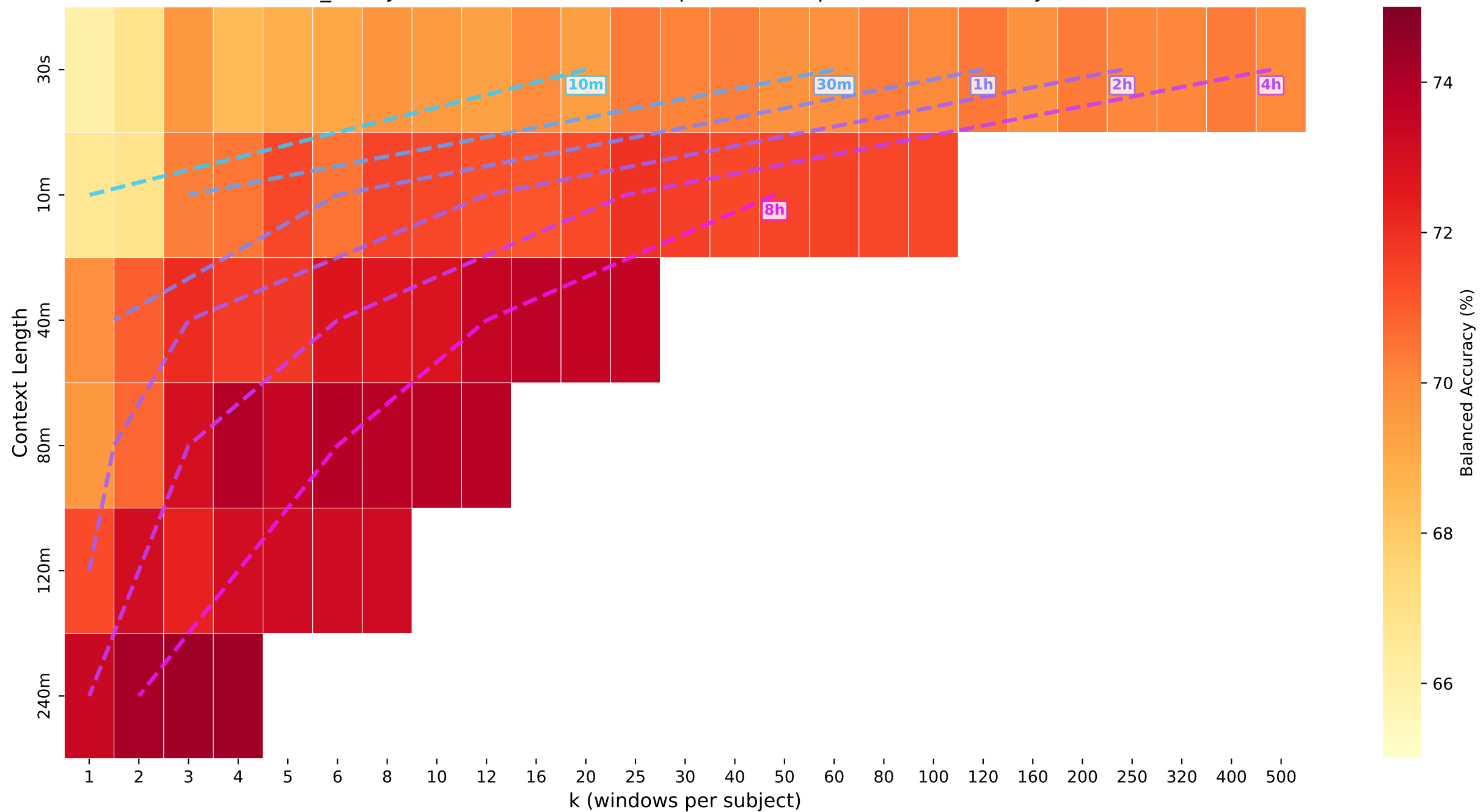
bmi_binary · transformer — Iso-Compute Heatmap: Balanced Accuracy (%)
