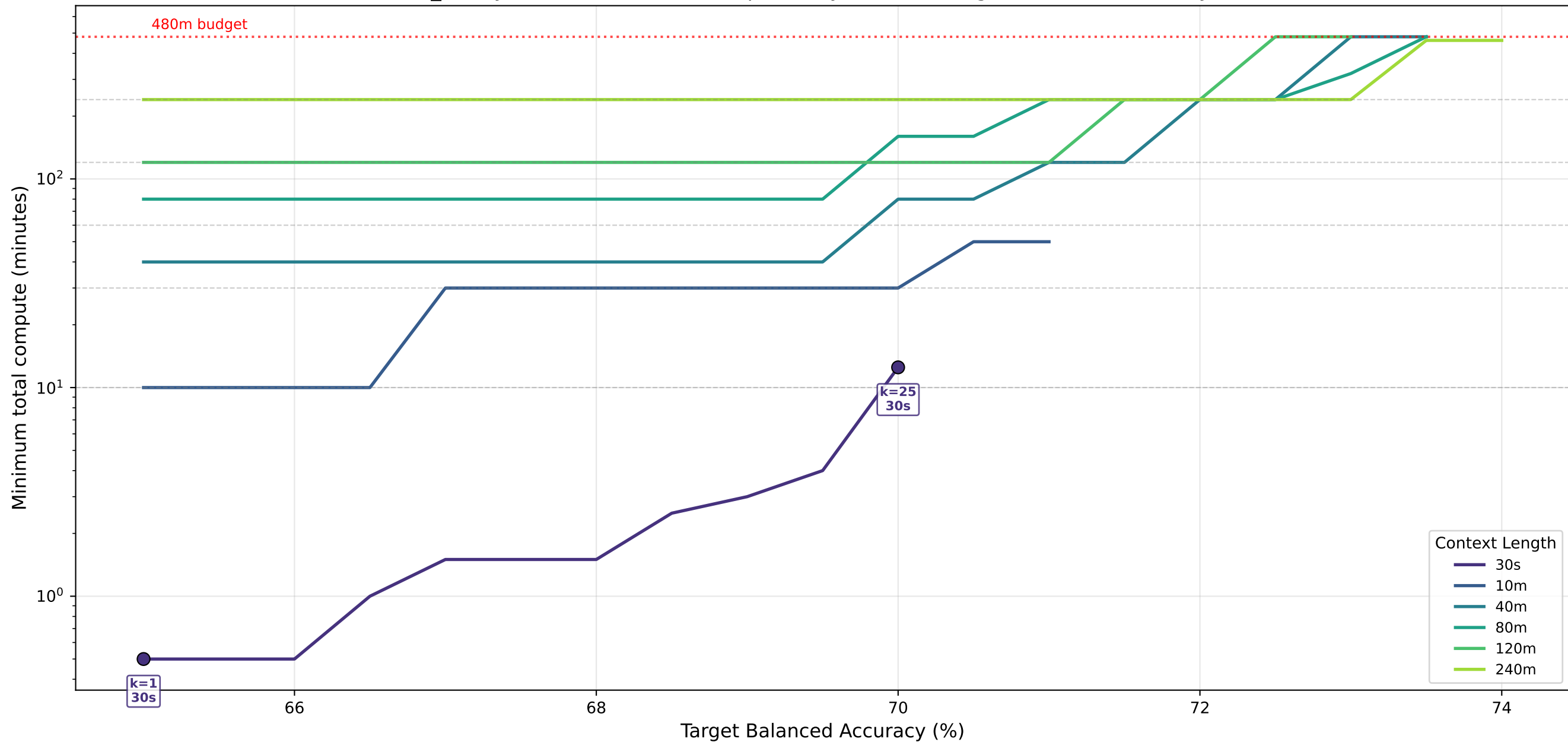
bmi_binary · transformer — Cheapest Way to Reach Target Balanced Accuracy (%)
