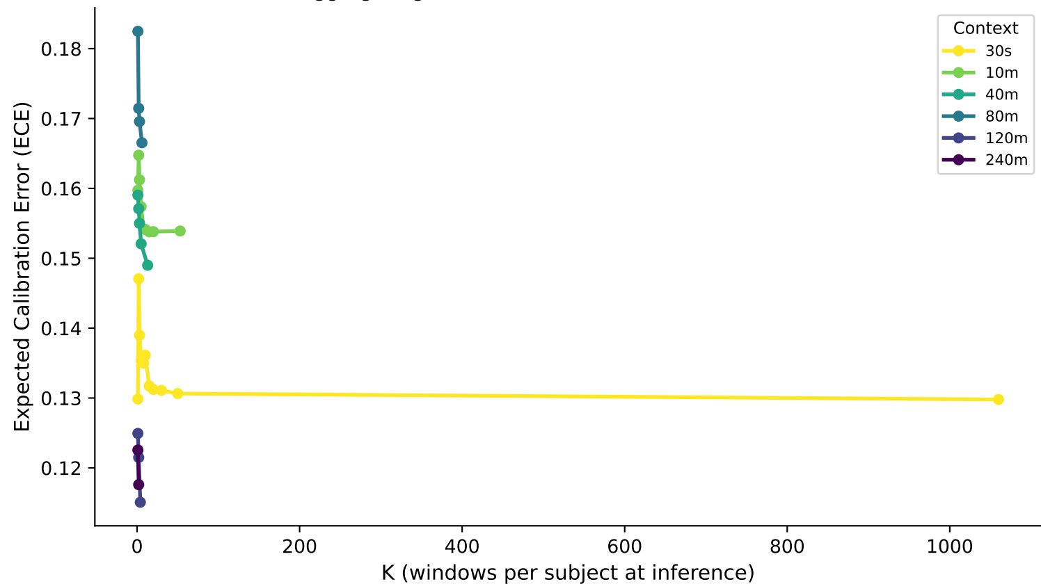
ECE vs K — bmi_binary (TRANSFORMER) Aggregating more windows reduces calibration error
