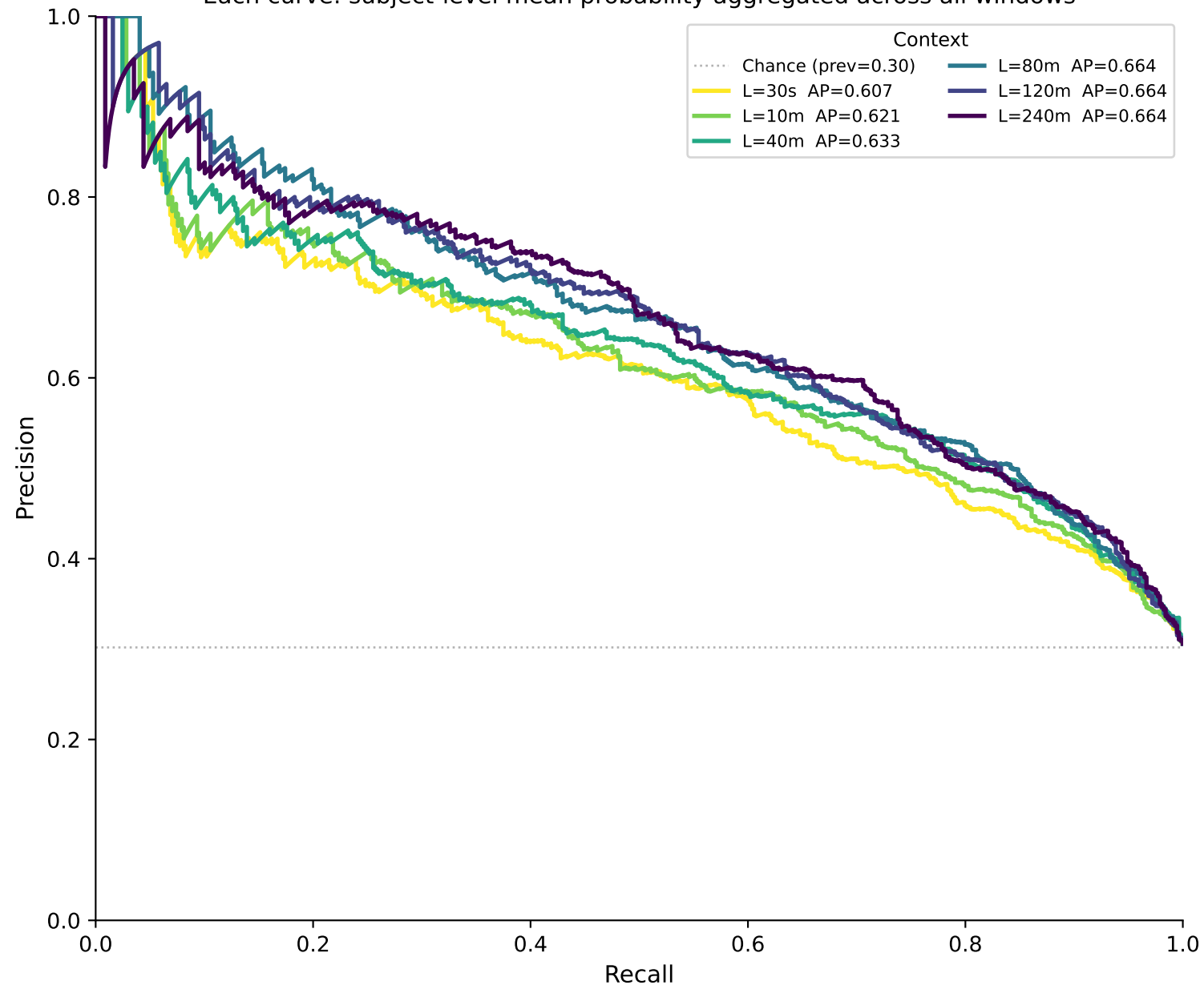
Precision-Recall Curves — bmi_binary (TRANSFORMER) K=all Each curve: subject-level mean probability aggregated across all windows
