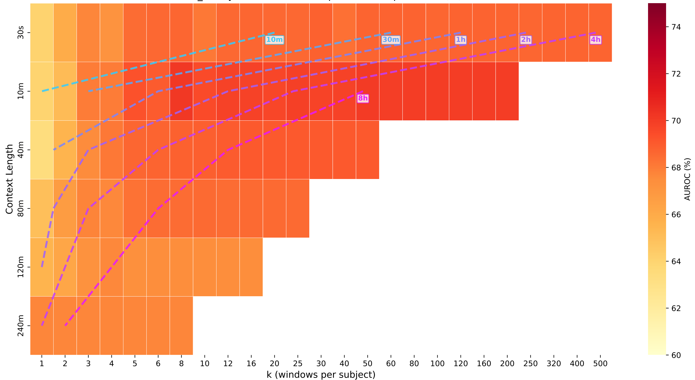
cvd_binary · lstm — Iso-Compute Heatmap: AUROC (%)
