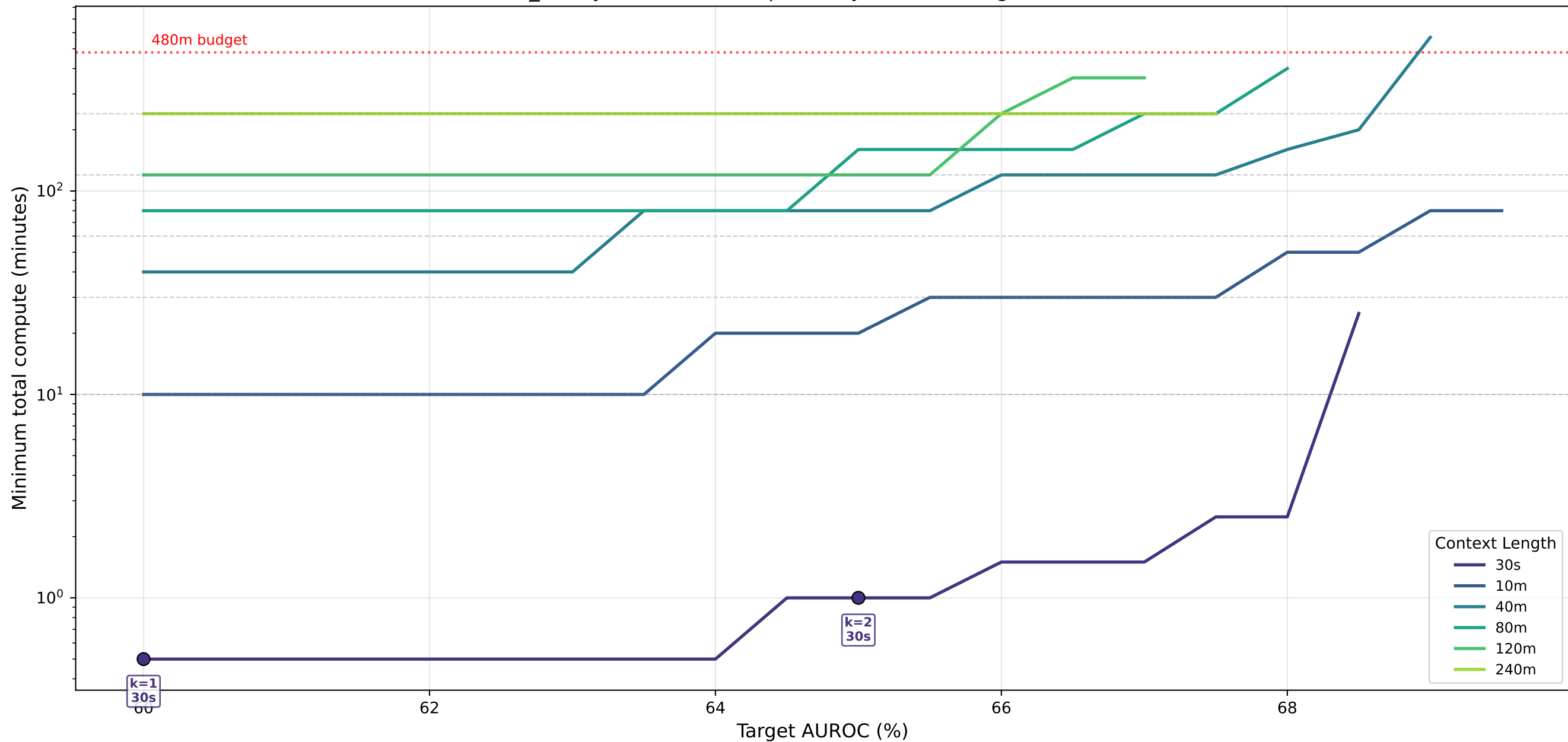
cvd_binary · lstm — Cheapest Way to Reach Target AUROC (%)
