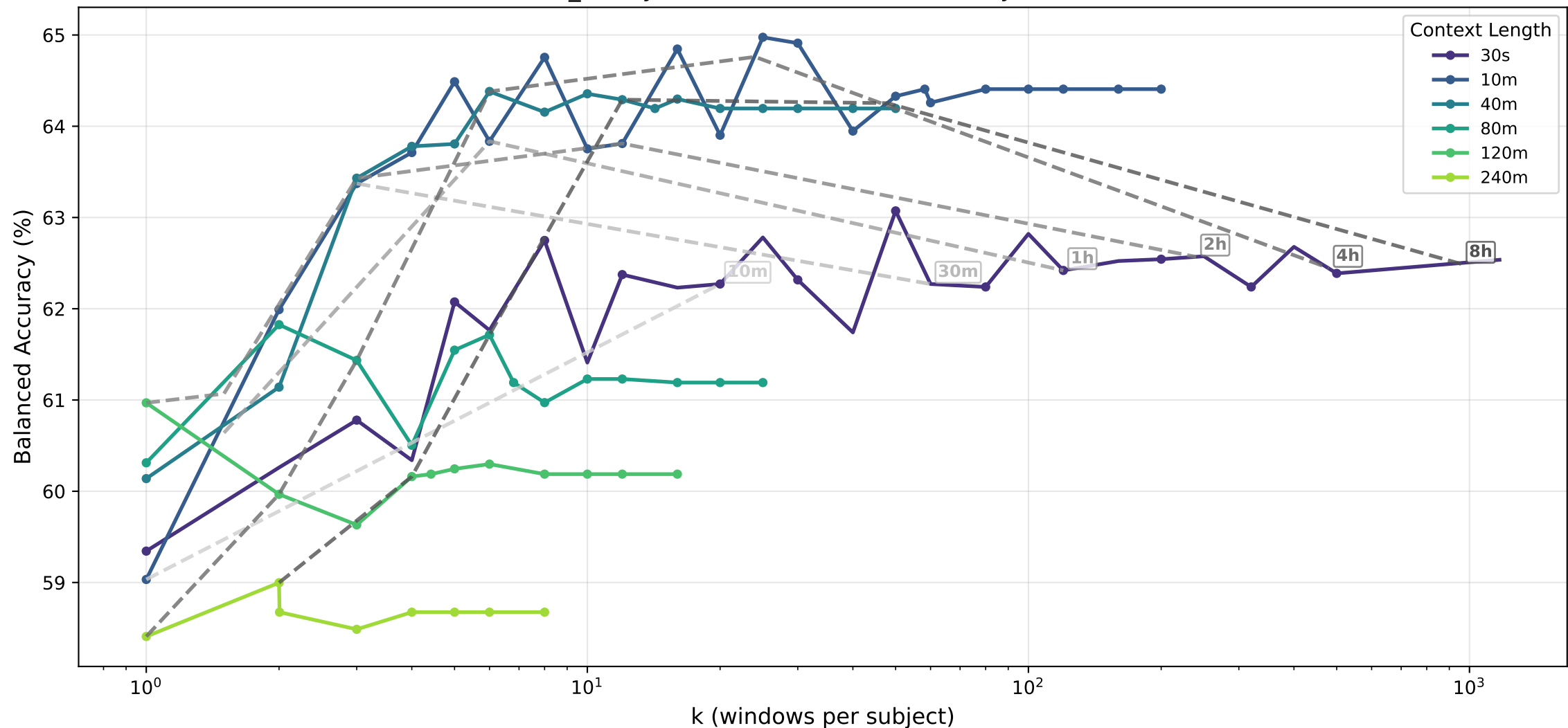
cvd_binary · lstm — Balanced Accuracy (%) vs k
