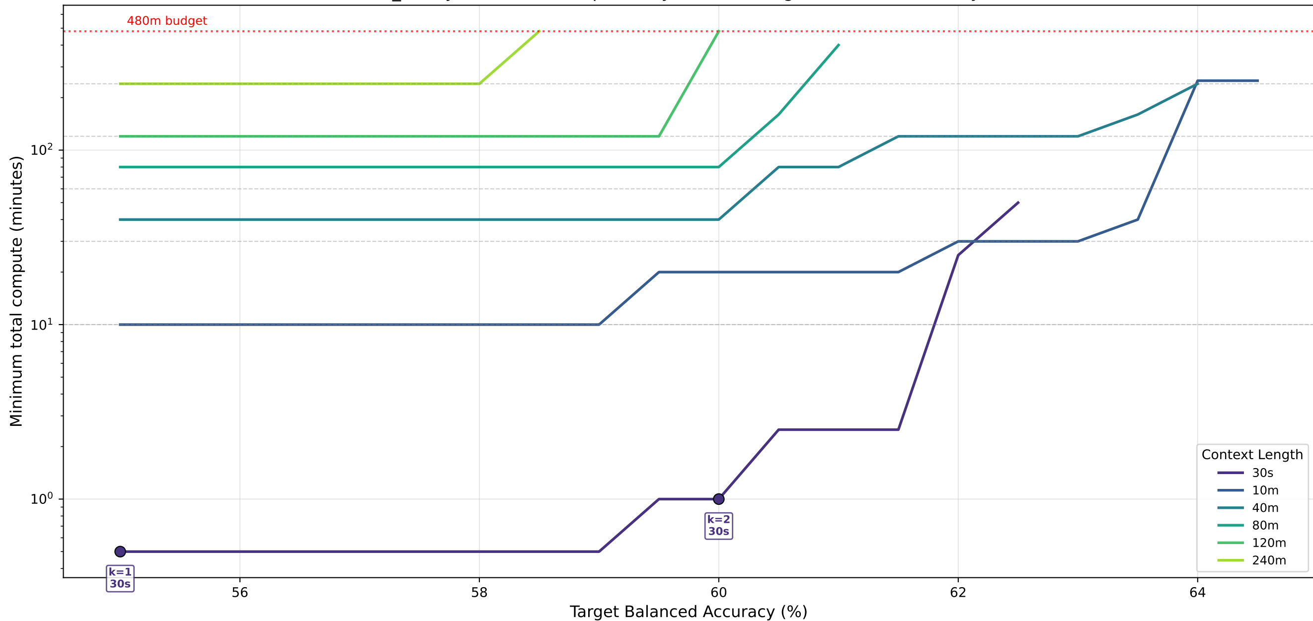
cvd_binary · lstm — Cheapest Way to Reach Target Balanced Accuracy (%)
