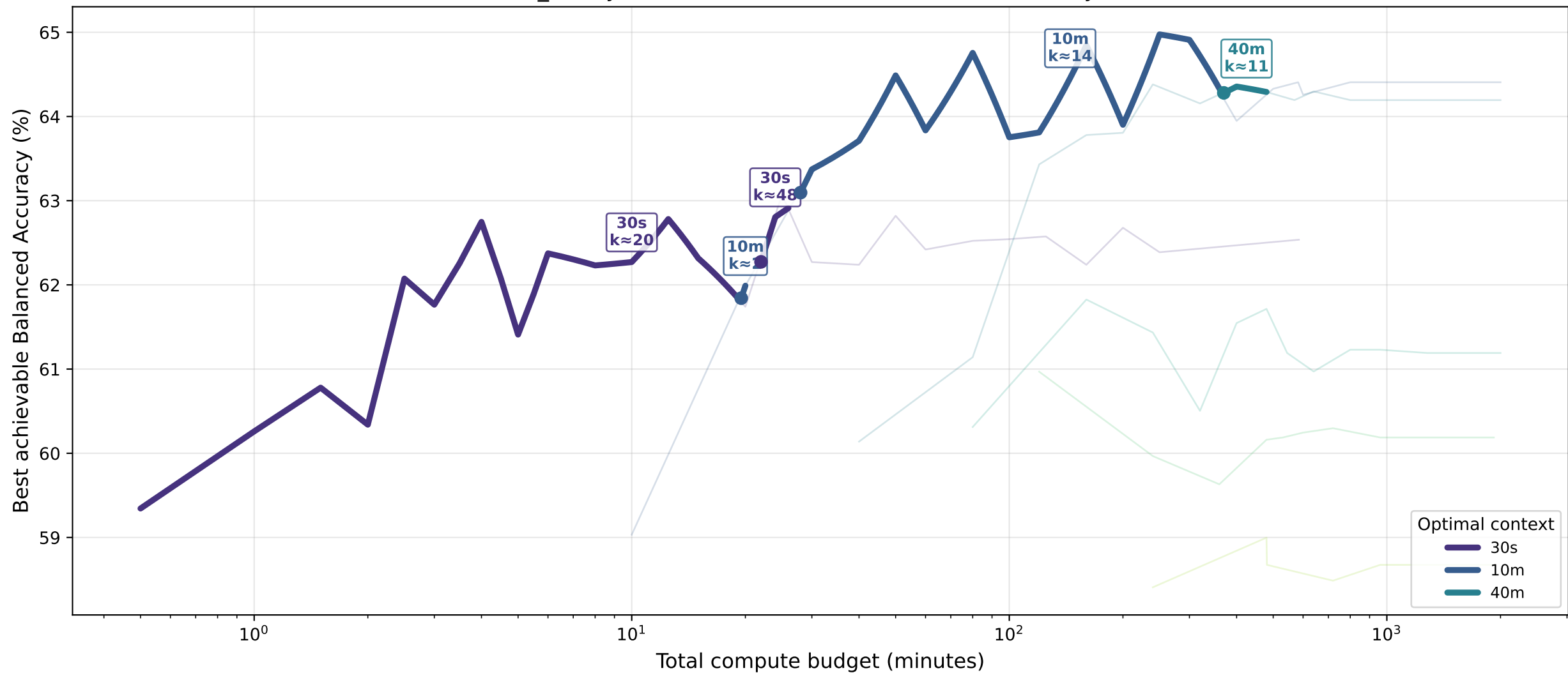
cvd_binary · lstm — Pareto Front: Balanced Accuracy (%)
