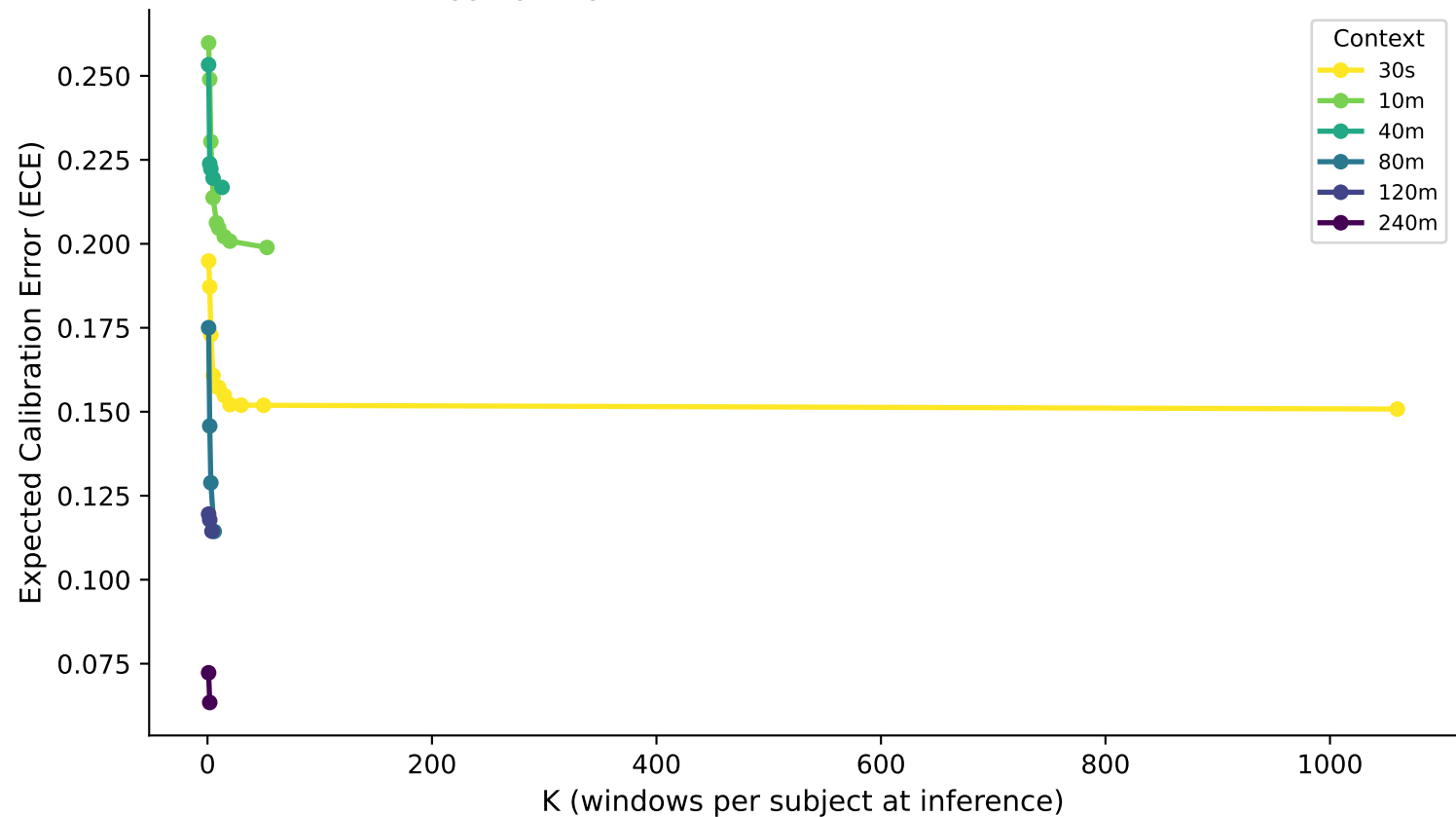
ECE vs K — cvd_binary (LSTM) Aggregating more windows reduces calibration error
