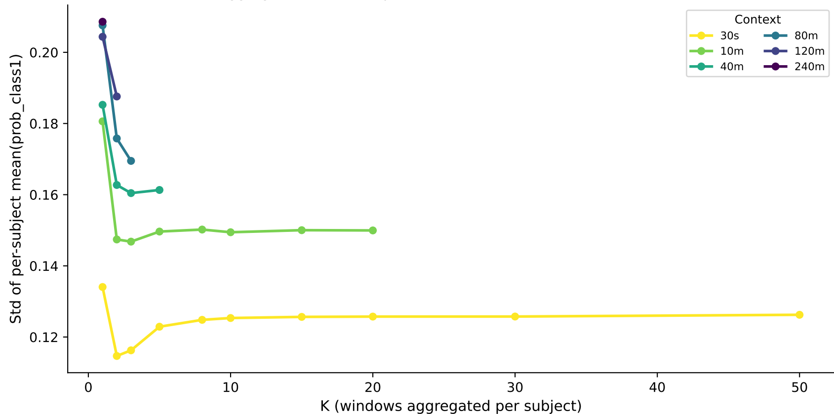
Prediction Variance vs K — cvd_binary (LSTM) Aggregation stabilises predictions (lower std = more consistent)
