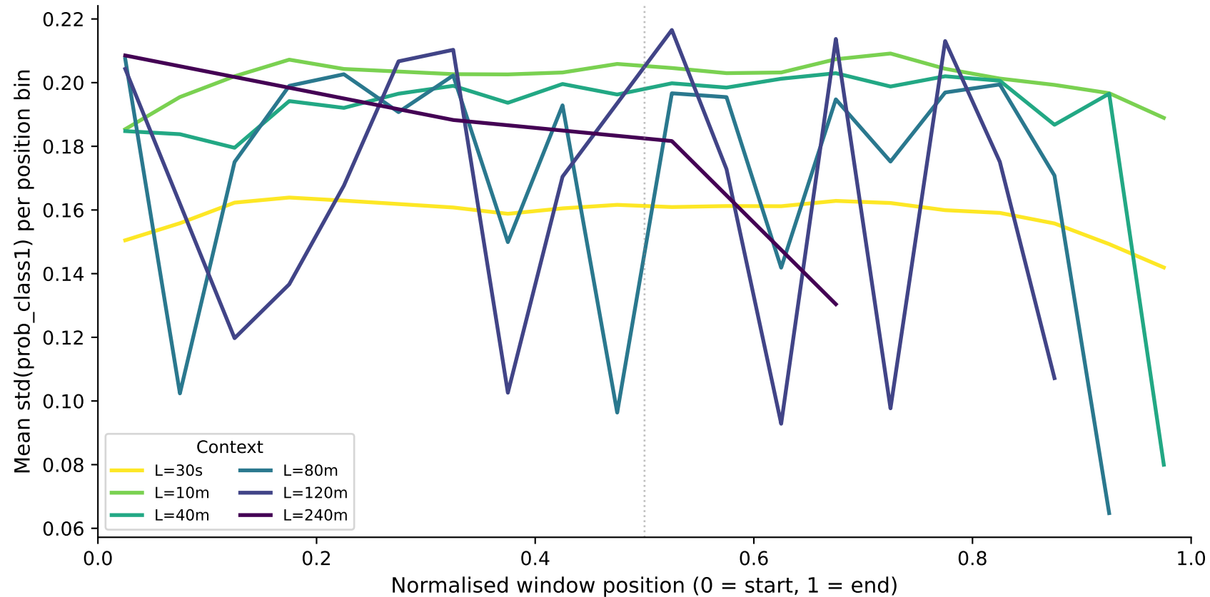
Prediction Variance vs Night Position — cvd_binary (LSTM) Lower variance = position-independent predictions (longer context may flatten this)
