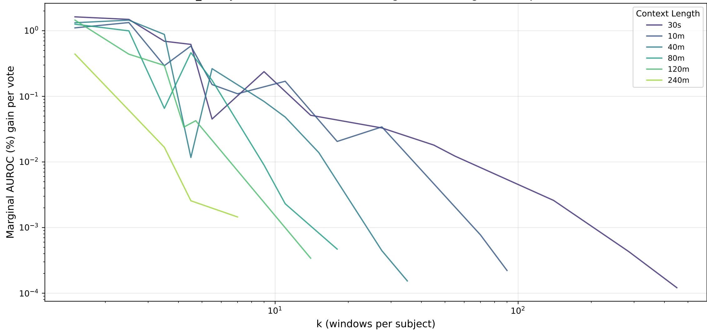
cvd_binary · transformer — Diminishing Returns: Marginal Gain per Vote
