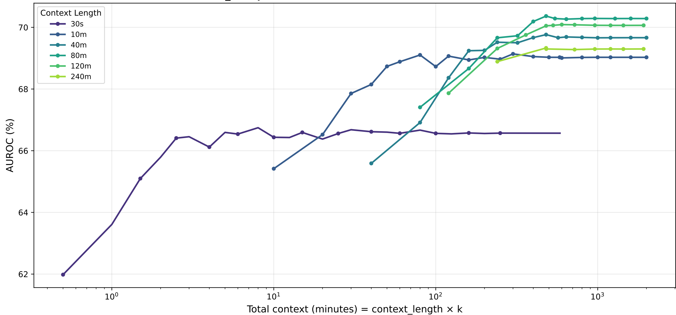
cvd_binary · transformer — AUROC (%) vs Total Context
