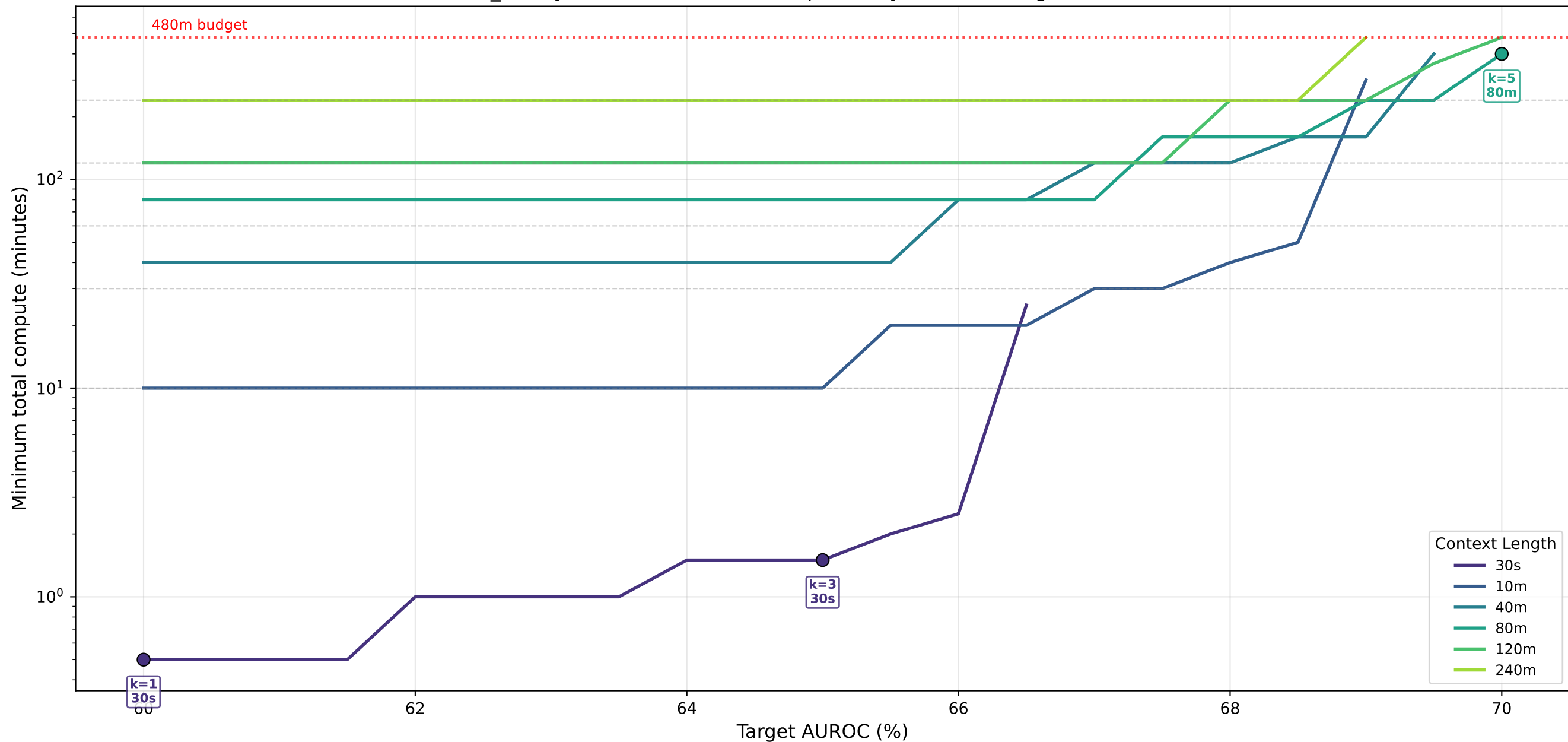
cvd_binary · transformer — Cheapest Way to Reach Target AUROC (%)
