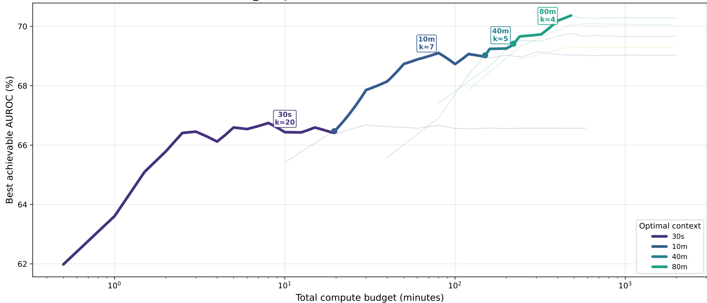
cvd_binary · transformer — Pareto Front: AUROC (%)
