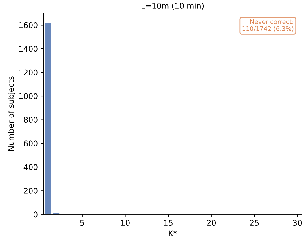
K* Distribution — cvd_binary (TRANSFORMER) K* = minimum windows for correct classification (reps=20)
