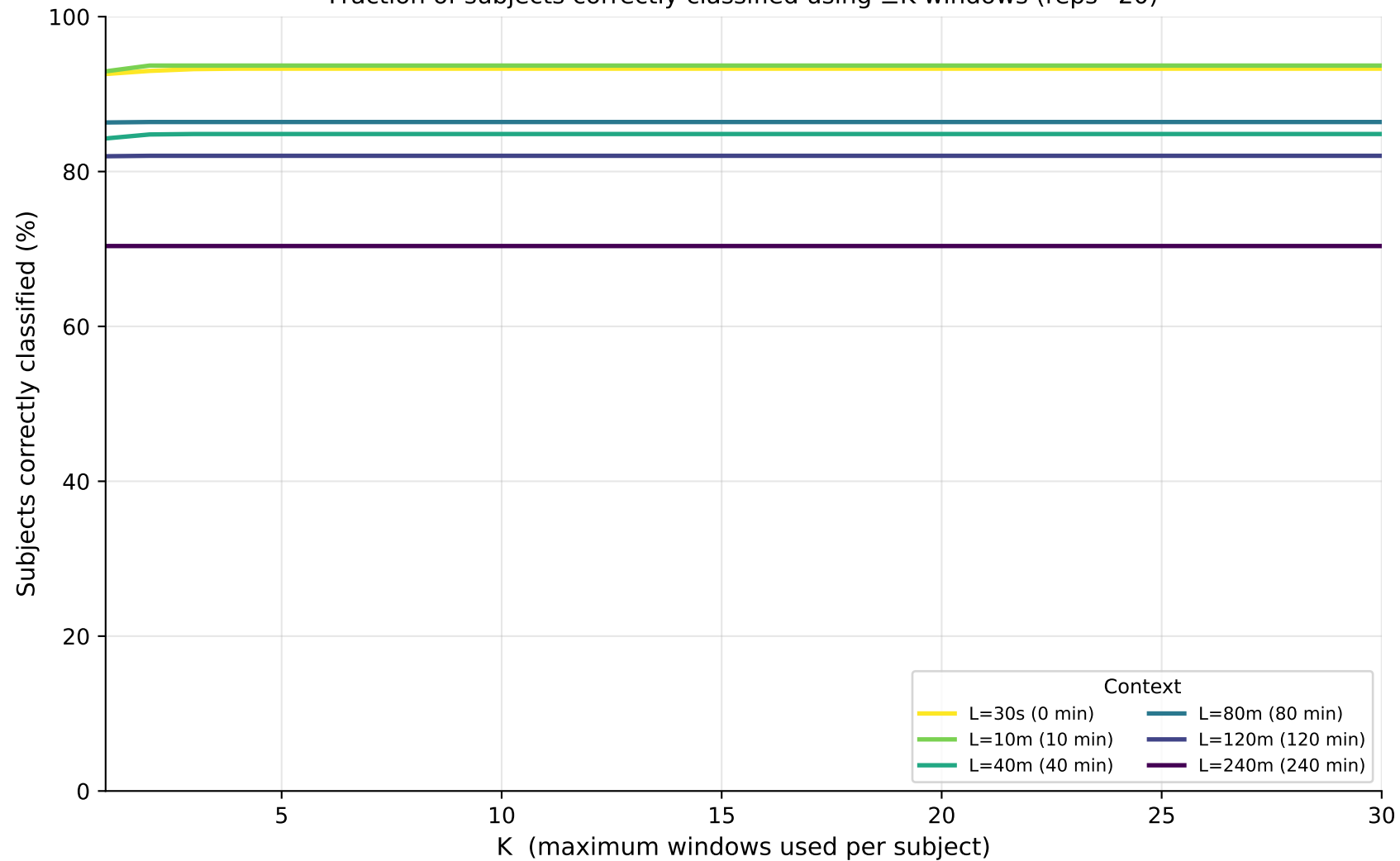
Coverage Curves — cvd_binary (TRANSFORMER) Fraction of subjects correctly classified using \leq K windows (reps=20)
