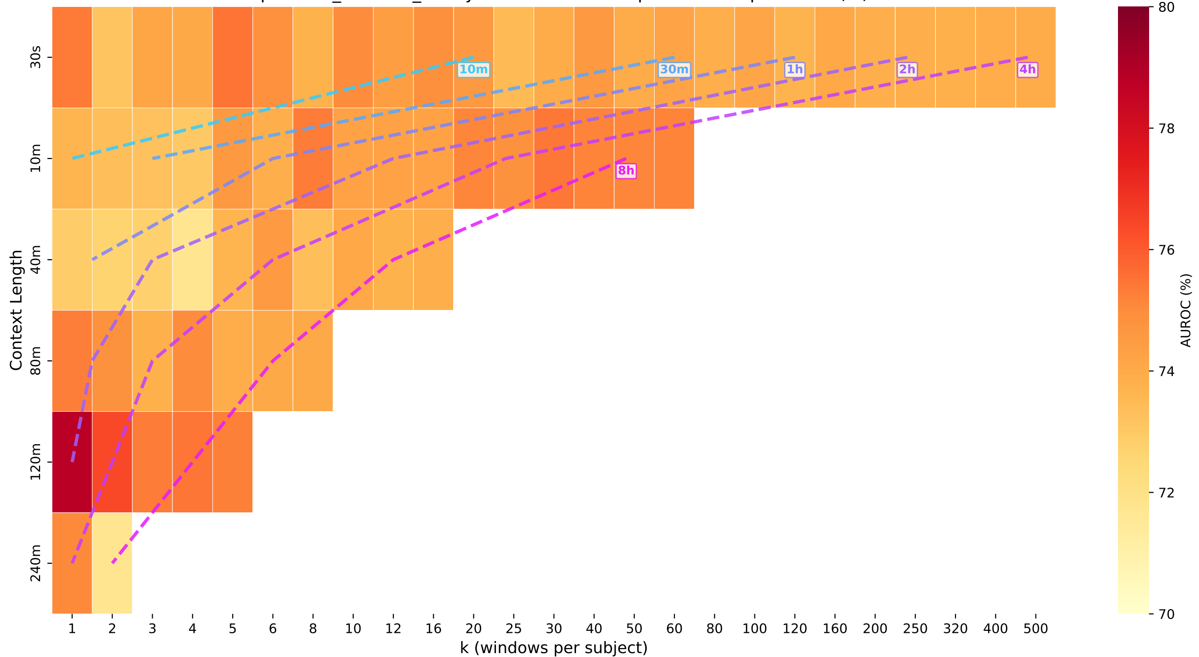
depression_extreme_binary · lstm — Iso-Compute Heatmap: AUROC (%)
