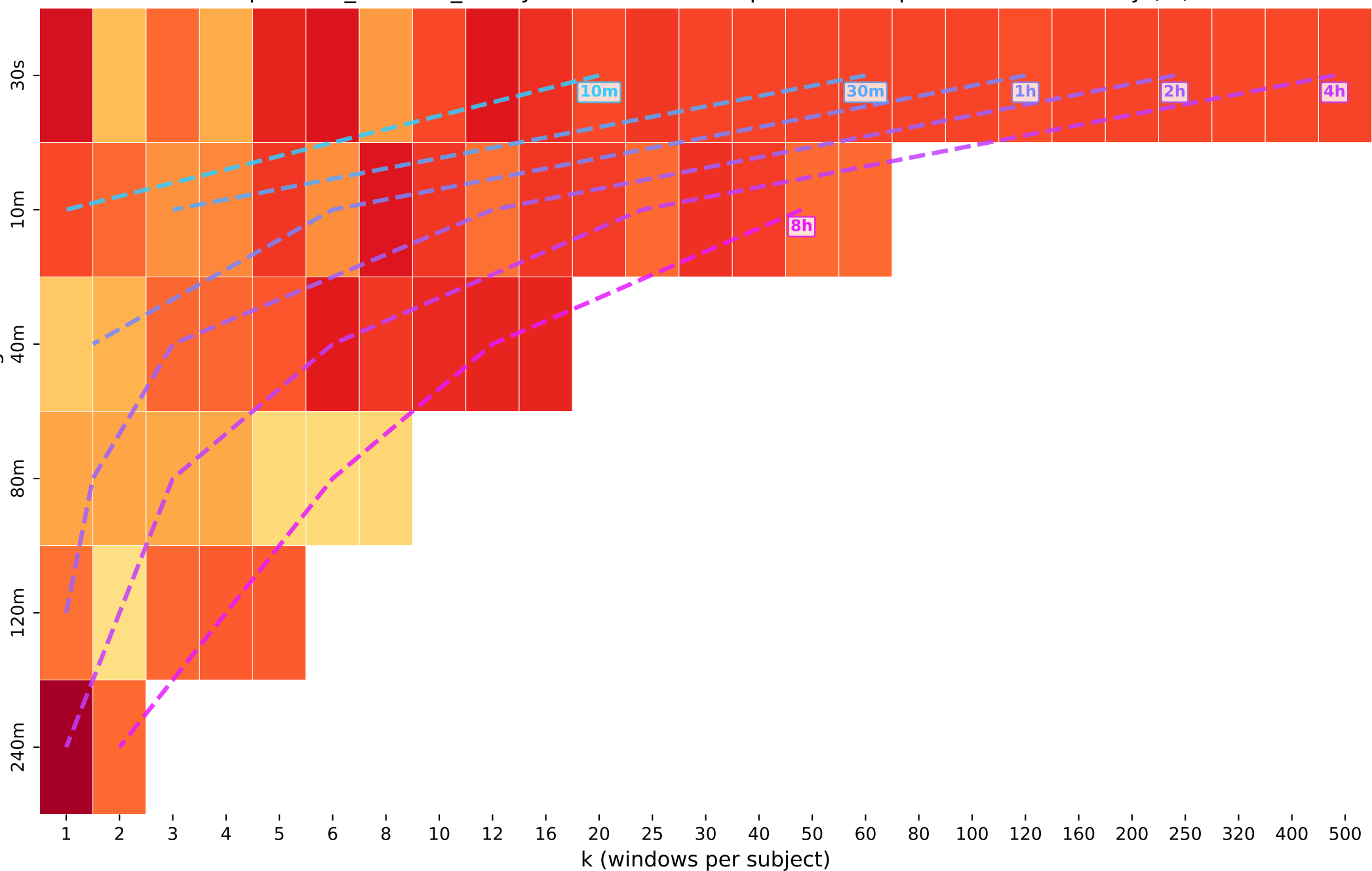
depression_extreme_binary · lstm — Iso-Compute Heatmap: Balanced Accuracy (%)
