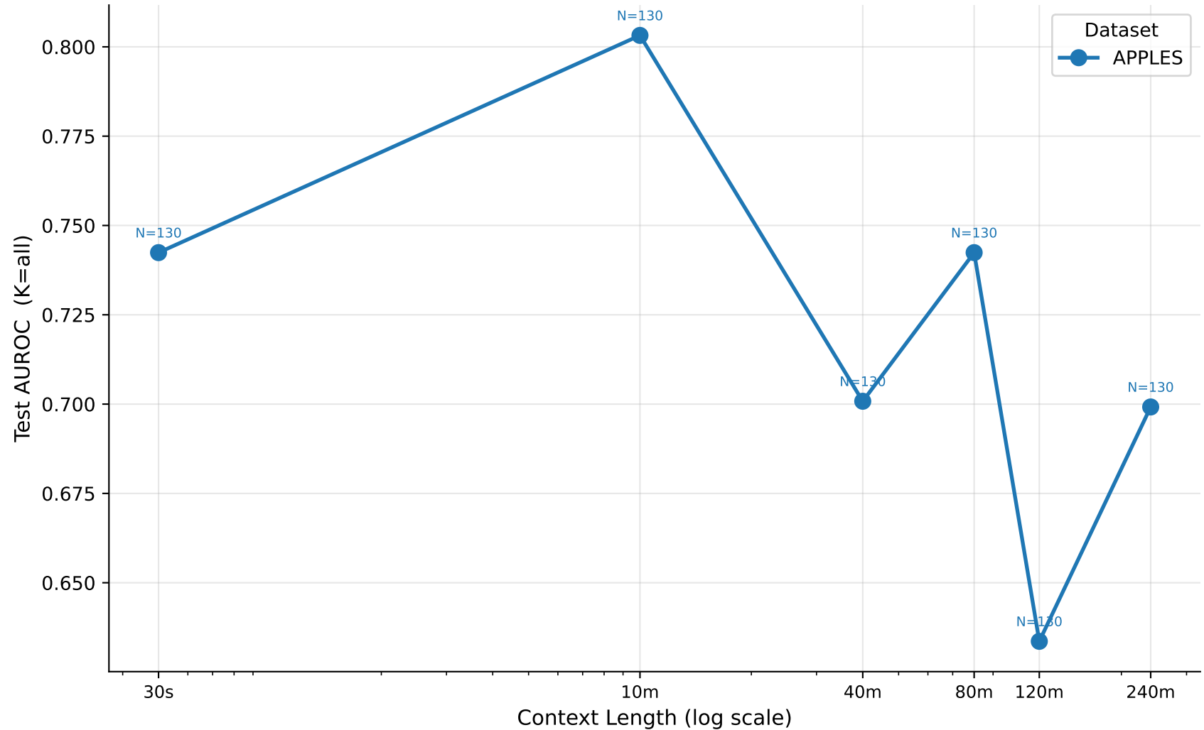
Cohort-Stratified Saturation — depression_extreme_binary (LSTM) Does the context saturation result hold across each dataset independently?
