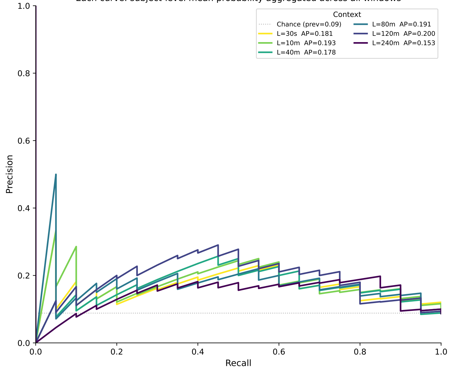
Precision-Recall Curves — depression_extreme_binary (LSTM) K=all Each curve: subject-level mean probability aggregated across all windows
