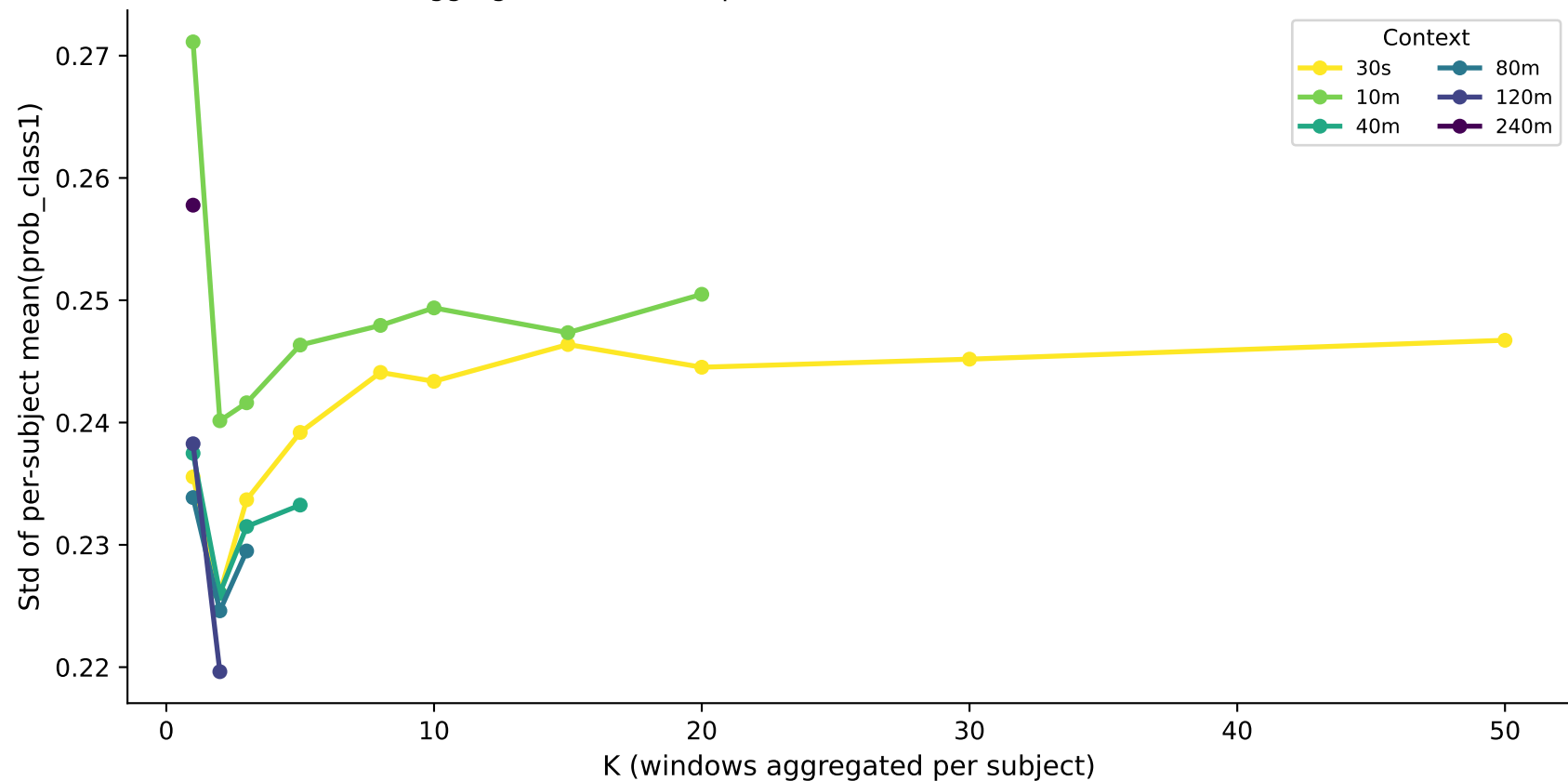
Prediction Variance vs K — depression_extreme_binary (LSTM) Aggregation stabilises predictions (lower std = more consistent)
