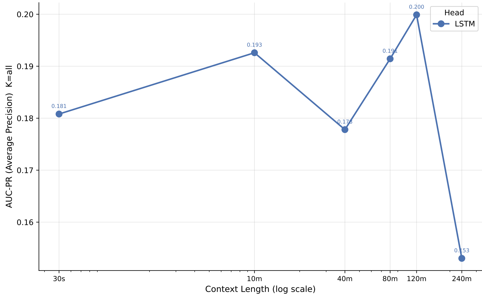
AUC-PR vs Context Length — depression_extreme_binary Does precision-recall performance saturate like AUROC?
