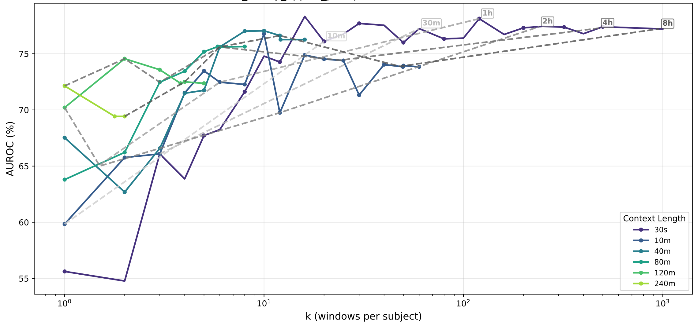
osa_binary_apples_postqc · lstm — AUROC (%) vs k
