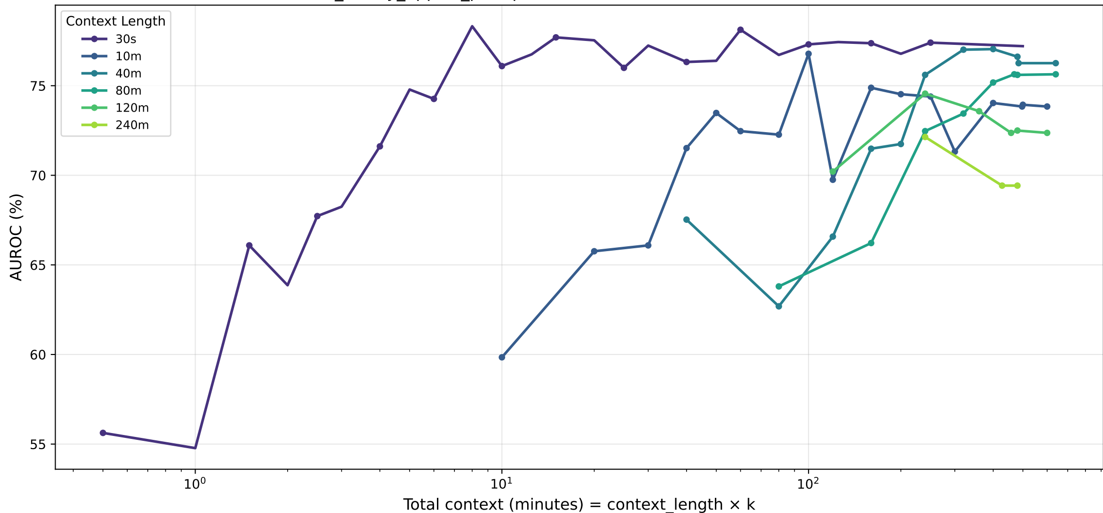
osa_binary_apples_postqc · lstm — AUROC (%) vs Total Context
