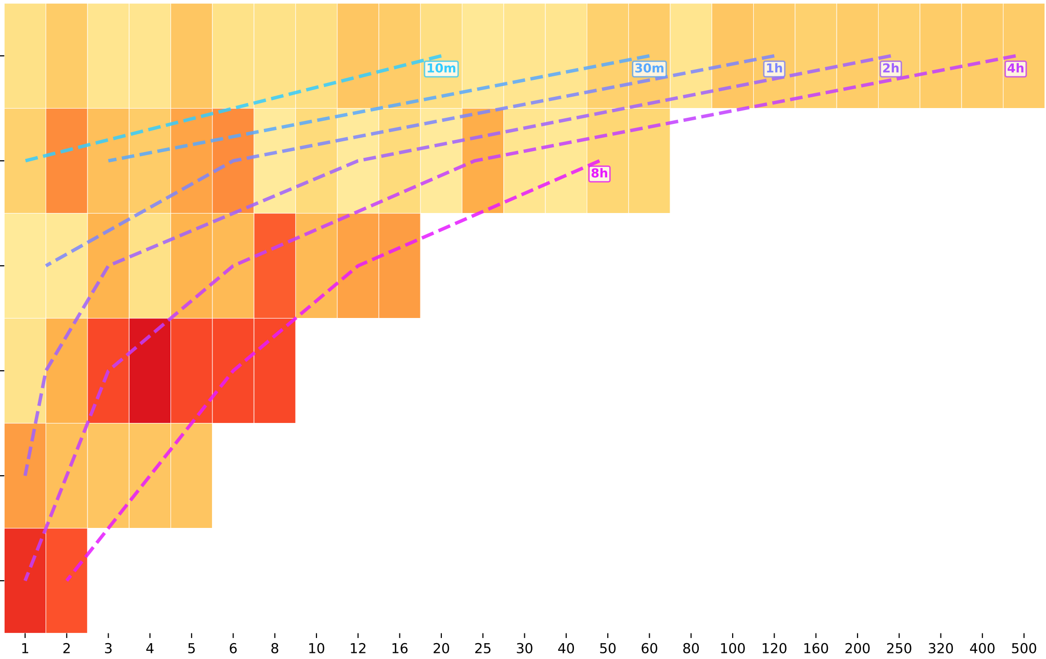
osa_binary_apples_postqc · lstm — Iso-Compute Heatmap: Balanced Accuracy (%)
