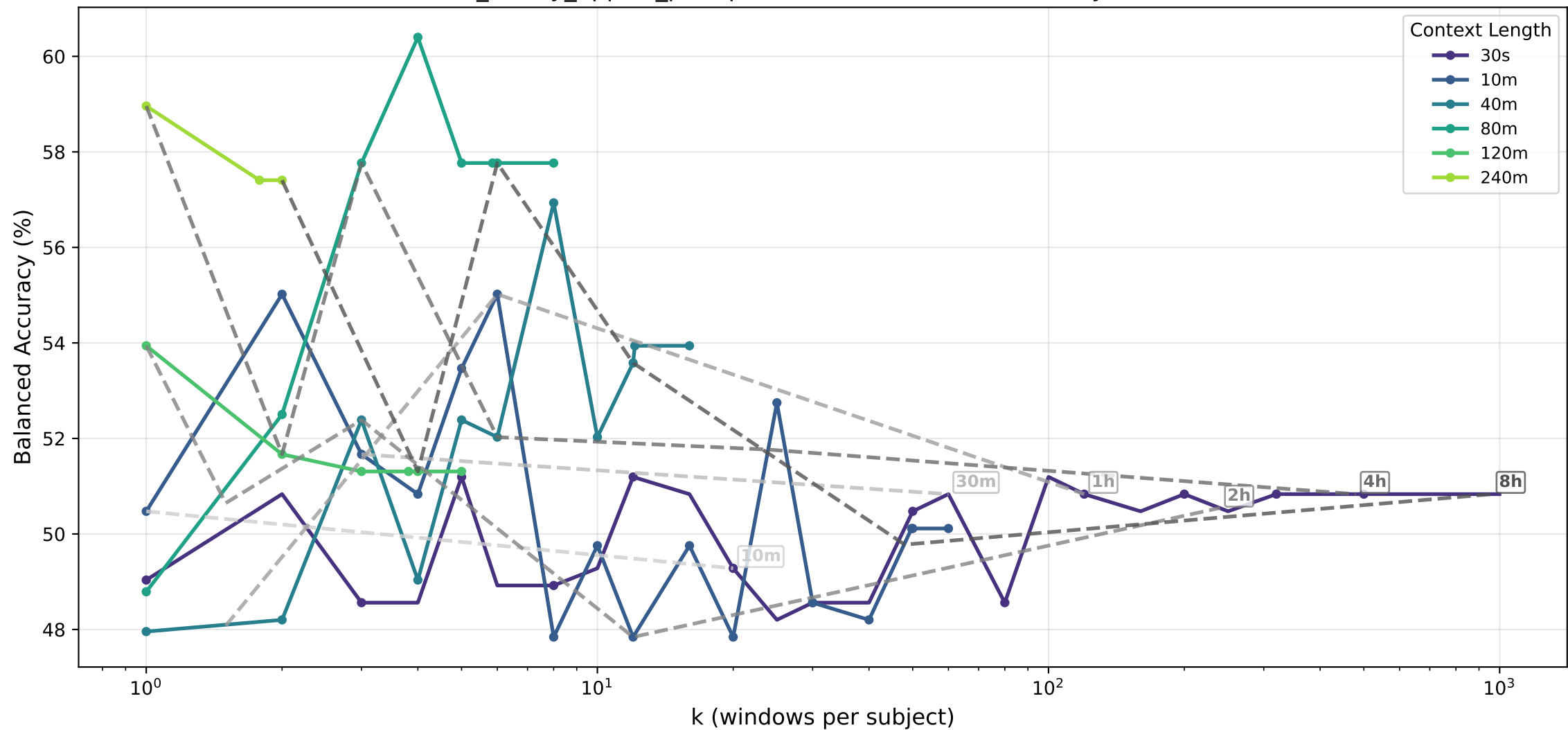
osa_binary_apples_postqc · lstm — Balanced Accuracy (%) vs k
