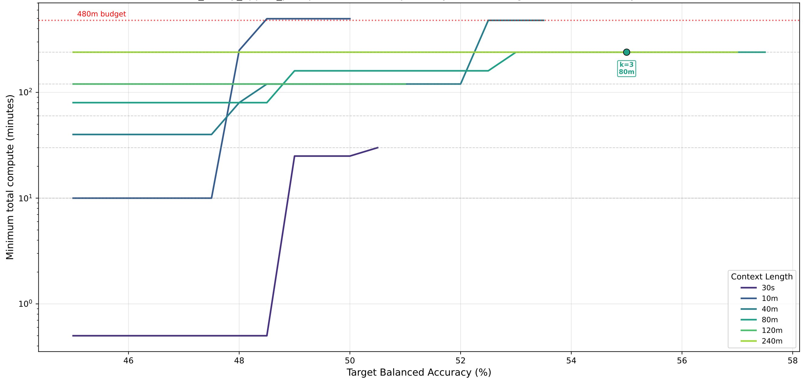
osa_binary_apples_postqc · lstm — Cheapest Way to Reach Target Balanced Accuracy (%)
