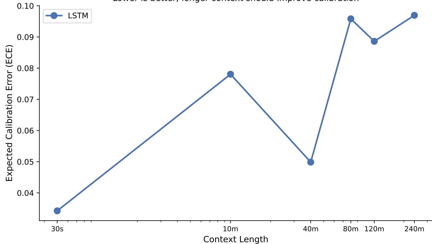
ECE vs Context Length — osa_binary_apples_postqc (K=10) Lower is better; longer context should improve calibration
