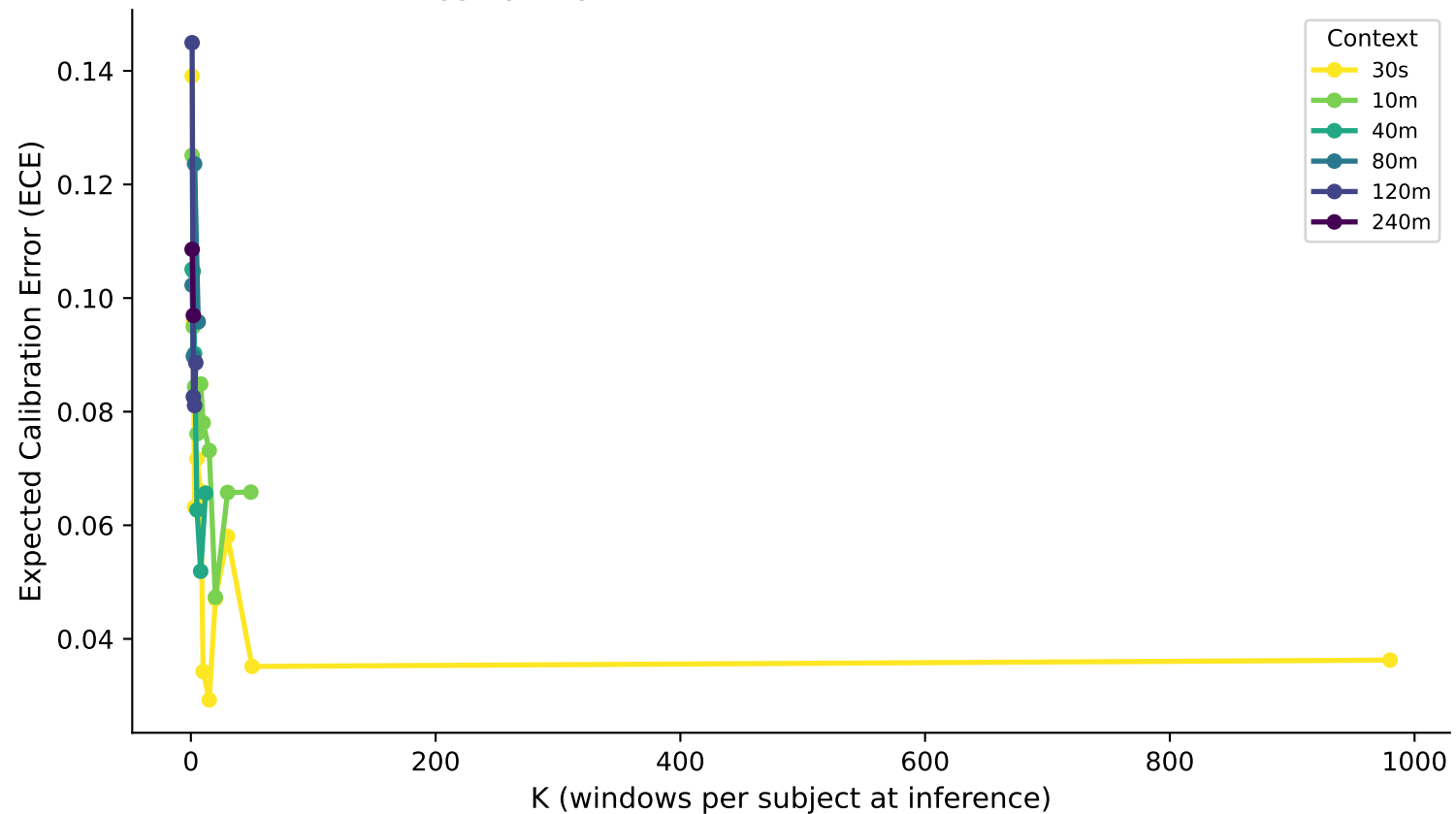
ECE vs K — osa_binary_apples_postqc (LSTM) Aggregating more windows reduces calibration error
