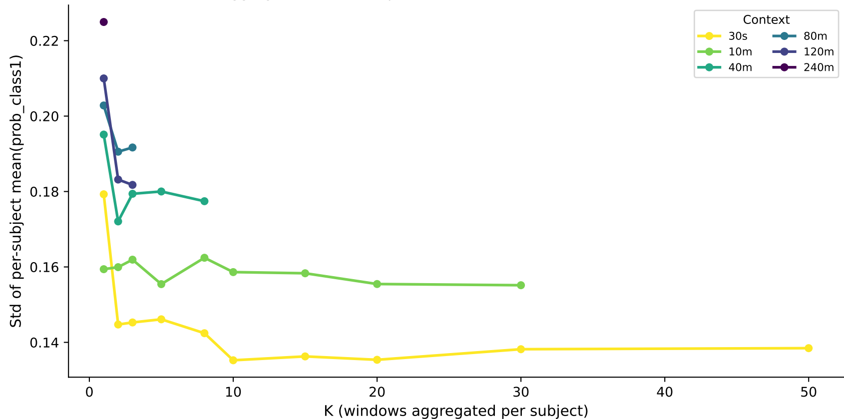
Prediction Variance vs K — osa_binary_apples_postqc (LSTM) Aggregation stabilises predictions (lower std = more consistent)
