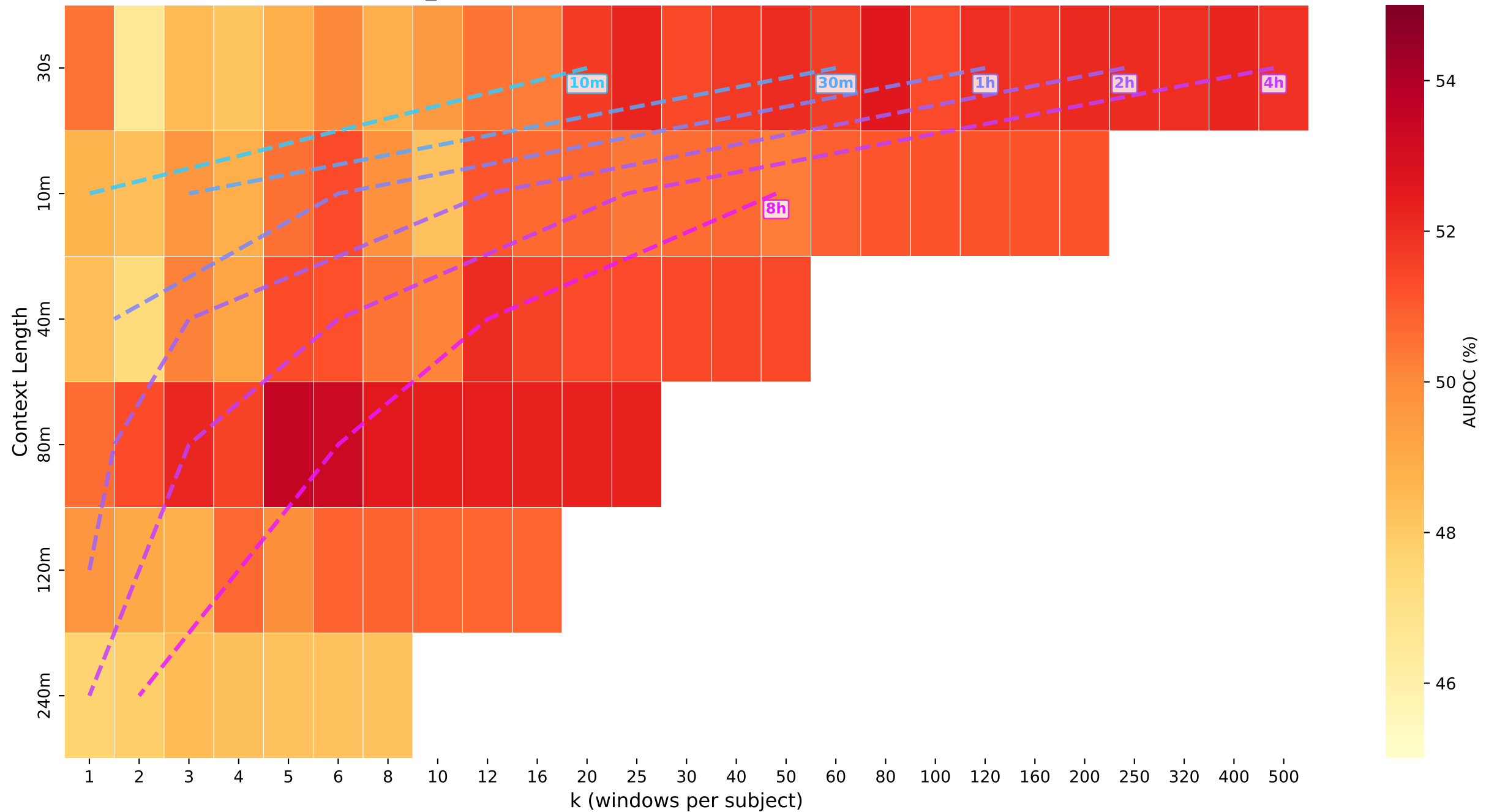
psqi_binary · lstm — Iso-Compute Heatmap: AUROC (%)
